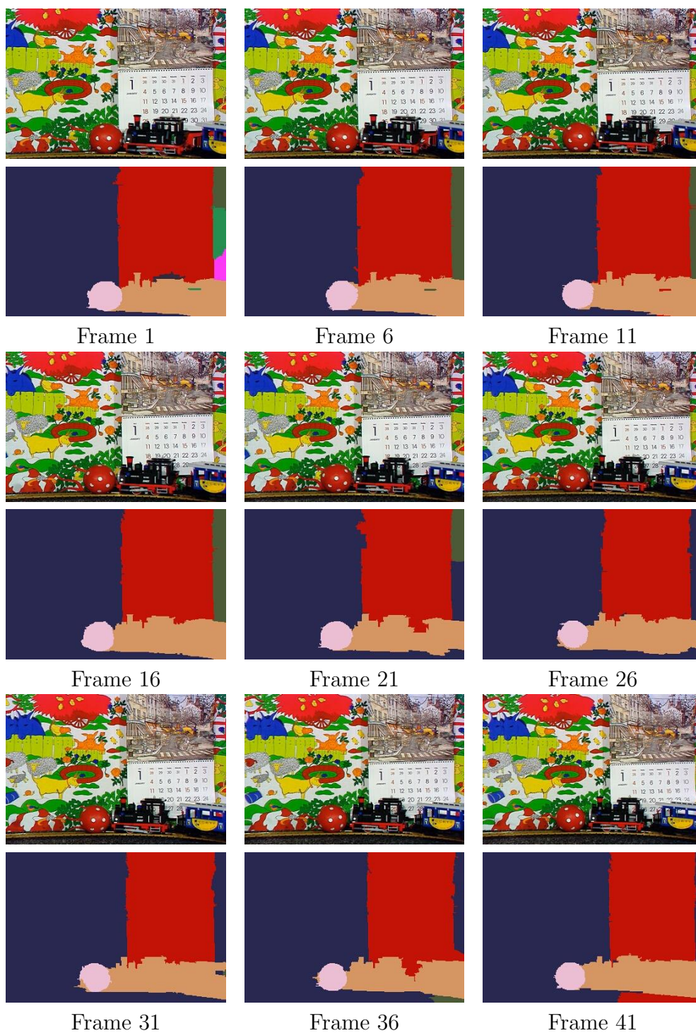
Figure 8.6: Motion segmentation.
