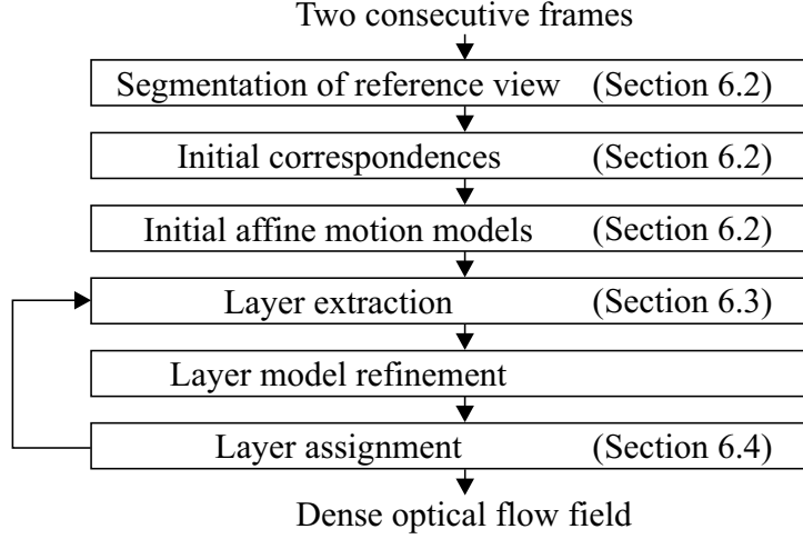
Figure 6.1: Algorithmic outline.
