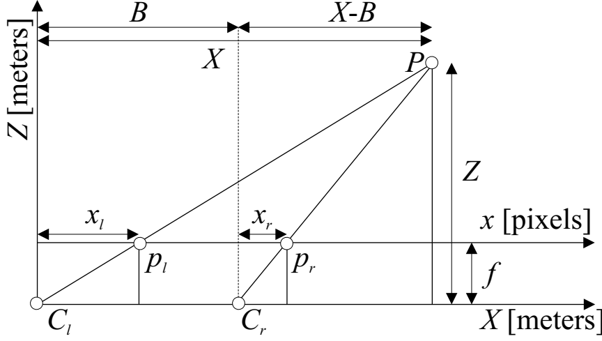
Figure 2.3: Reconstruction of the depth coordinate via triangulation.
