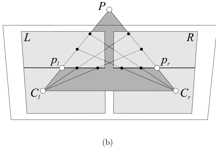
Figure 2.2: Epipolar geometry. (a) Epipolar lines for cameras in general positions and orientations. The matching point in one view must lie on the corresponding epipolar line in the other view. (b) Epipolar lines after epipolar rectification. Image planes lie in the same plane and x-axes are parallel to the baseline. The matching point in one view lies on the same horizontal scanline in the other image.
