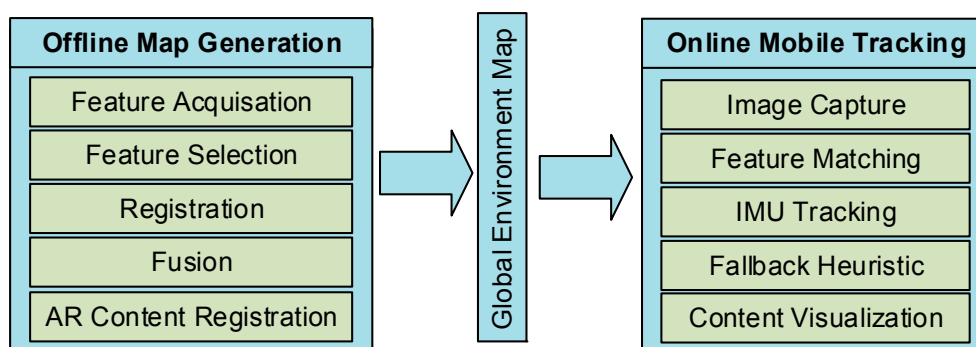
Figure 1. Developed packages for the HyMoTrack framework.
