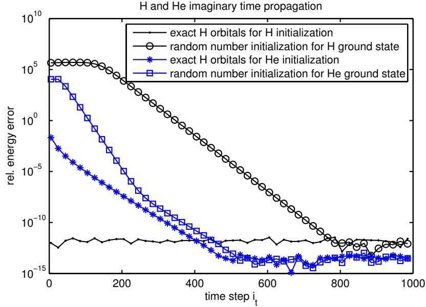
Figure 6.19: Convergence of the ground state energy approximation. Energy error over time step i_t for imaginary time propagation of a hydrogen and a helium atom. Comparison of convergence between initialization with hydrogenic orbitals and with random numbers, r_{\max} = 100 , \Delta r_H = \frac{1}{400} , \Delta r_{He} = \frac{1}{100} , n_t = 1000 steps, \Delta t = \frac{1}{16} .
