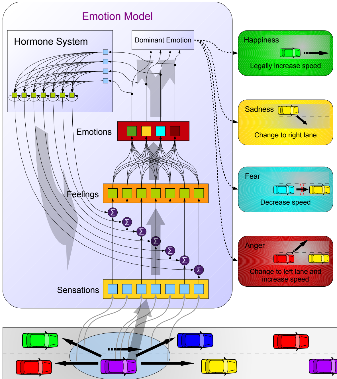
Figure 3.3: SAD driving
