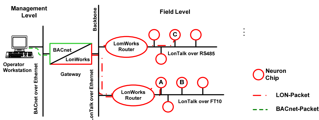
Figure 15: Communication with gateways
