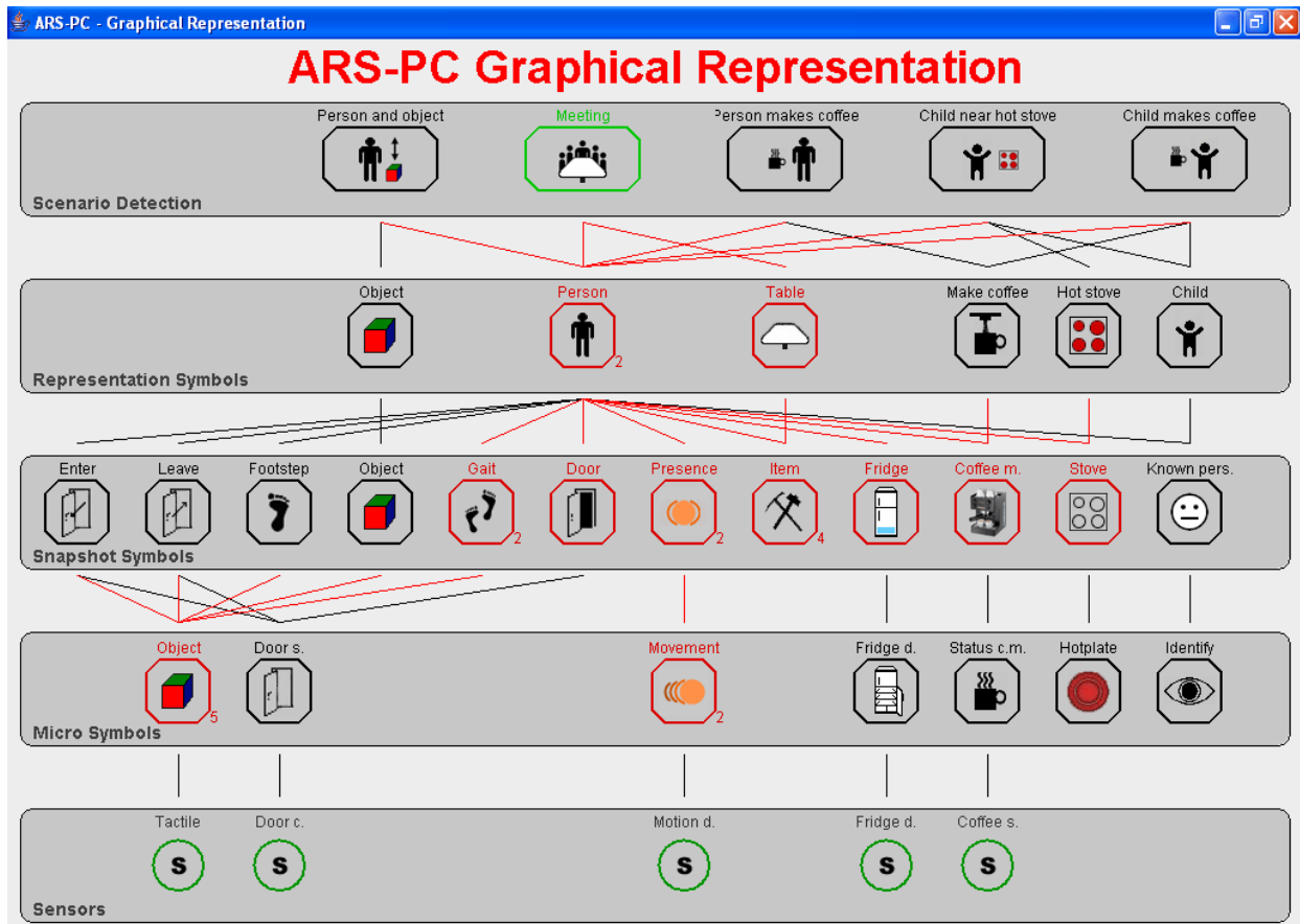
Figure 99: Screenshot of logical view of the symbols
