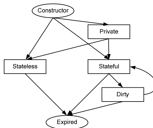
Figure 31: Lifecycle in SymbolNet
