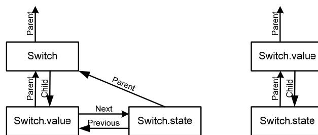
Figure 19: Mapping SNVT_switch to DPAL data points
