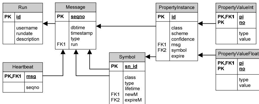
Figure 35: Sensor database tables
