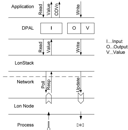
Figure 23: DPAL acts as CNP application without NVs
