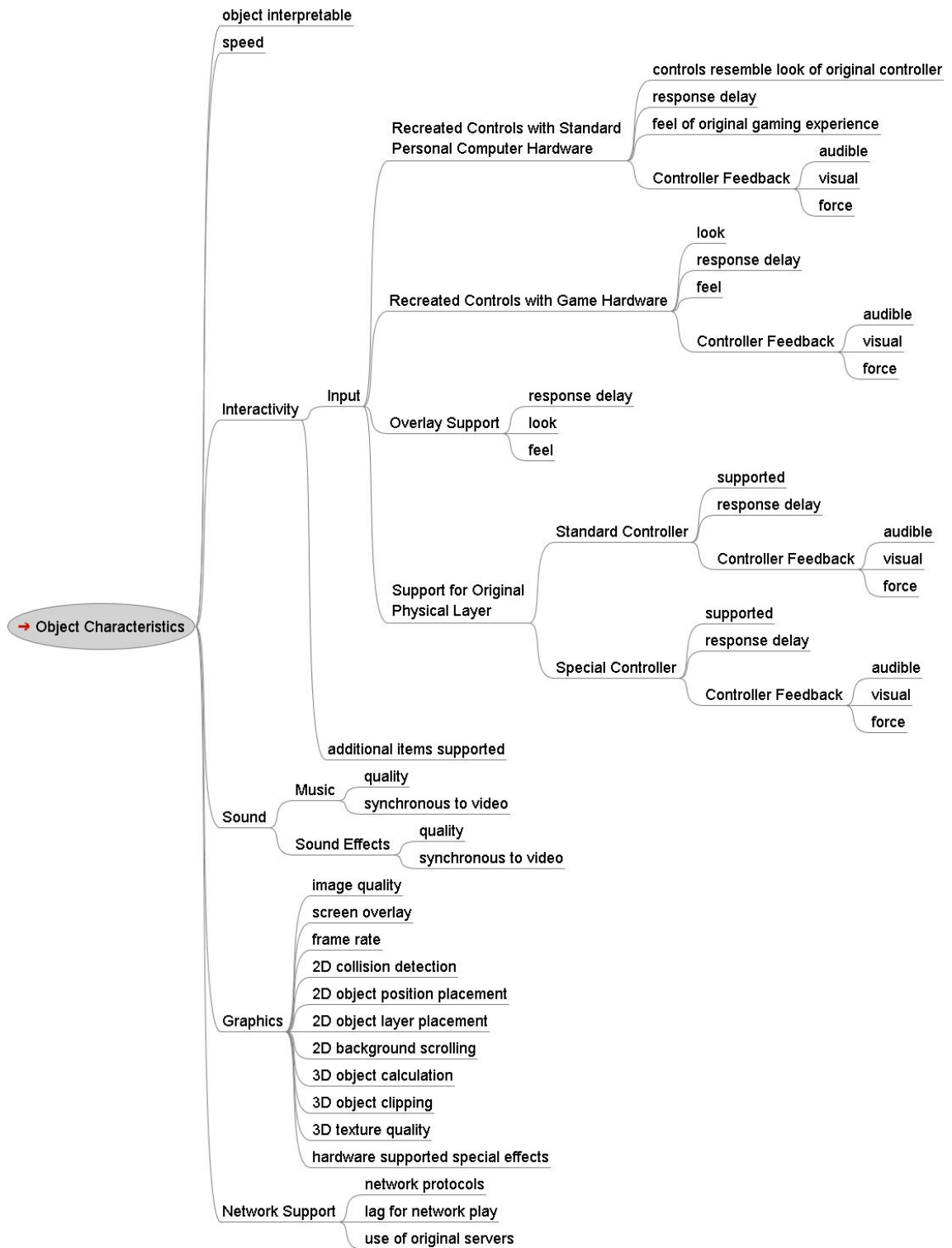
Figure 4.1: Object characteristics requirements sub tree.
