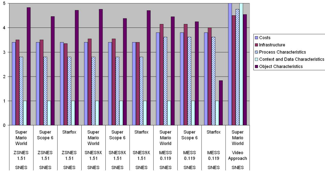
Figure 4.10: Aggregated results for the main categories in the requirements trees for Nintendo SNES preservation alternatives (weighted sum).
