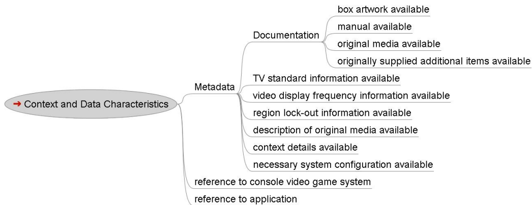
Figure 4.2: Context and data characteristics requirements sub tree.
