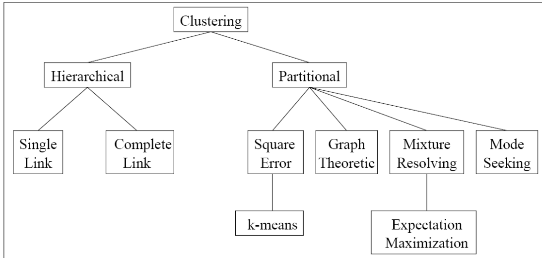
Figure 2.1: Classification of clustering approaches [Jain et al., 1999]
