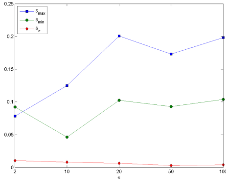
(a) \delta_{max} , \delta_{min} and \delta_{\sigma} of \Delta_{50} for varying \pi of the genre Classic
