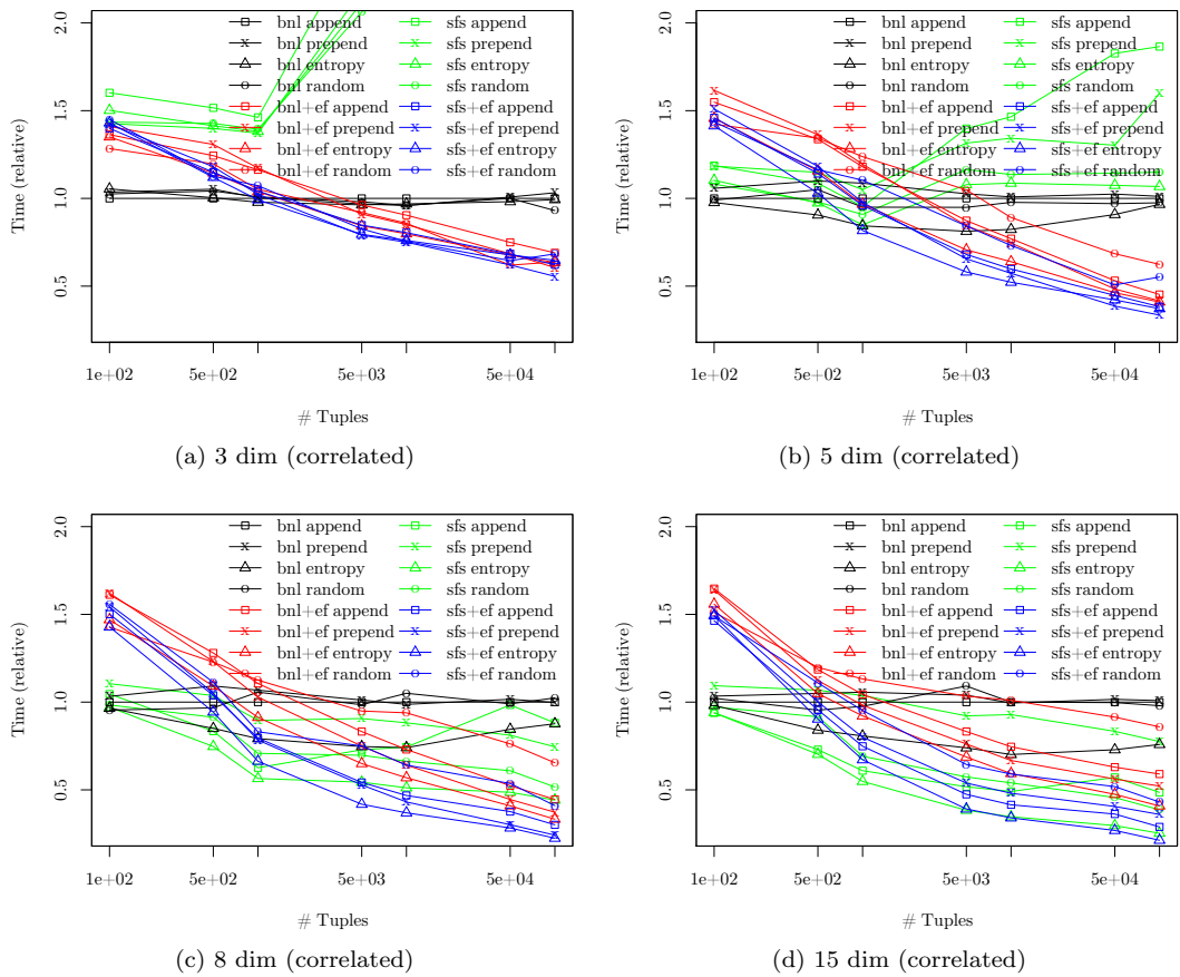
Figure 5.13: Comparing runtime for correlated datasets
