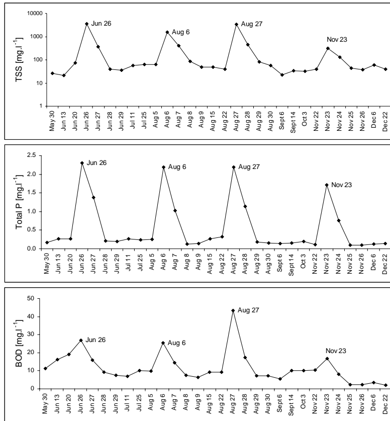
Figure 3. Storm induced clockwise hysteresis for TSS, total P and BOD
