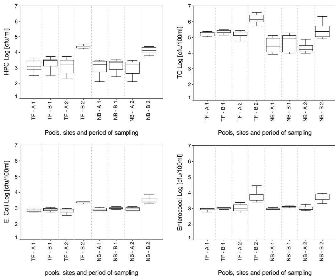
Figure 3: Box-whisker plots illustrating the site segregation capacity of the microbial indicators at Turkana Flats (TF) and Njoro Bridge (NB). Note a significant ( p < 0.05 ) increase in downstream levels during in-stream activities (TF-B2 & NB-B2). The legend in Fig. 2 gives a description of the box-whisker plot, the sites and the sampling period.
