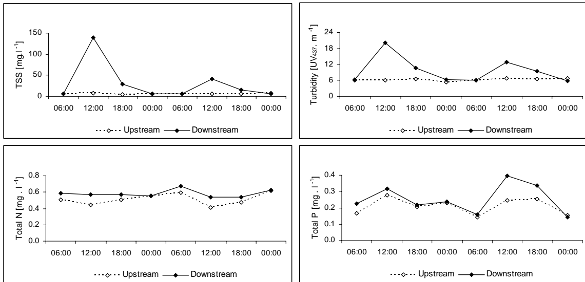
Figure 6. Diurnal transients provoked by in-stream activities on two consecutive days for TSS, Turbidity, TP and TN at Turkana Flats in dry weather (January–April)
