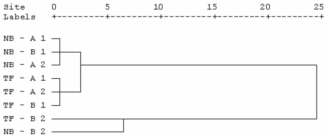
Figure 5. Dendrogram illustrating the average linkages between sites at Turkana Flats (TF) and Njoro Bridge (NB). Note in particular the segregation of the downstream sites during in-stream activities (TF – B2 & NB – B2). The legend in Fig. 2 gives a description of the sites and the period of sampling.
