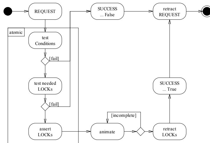
Figure 3.3: Environment activities for an Action REQUEST
