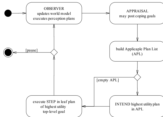
Figure 3.4: Activity Diagram: Agent Execution Cycle
