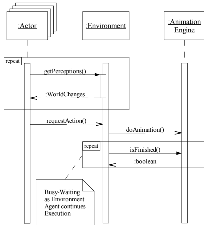
Figure 3.1: Sequence Diagram: Interaction of the Stage Threads
