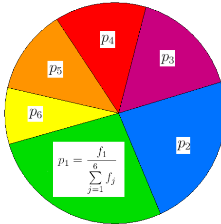
Figure 2.1: Schematic visualization of roulette wheel selection
