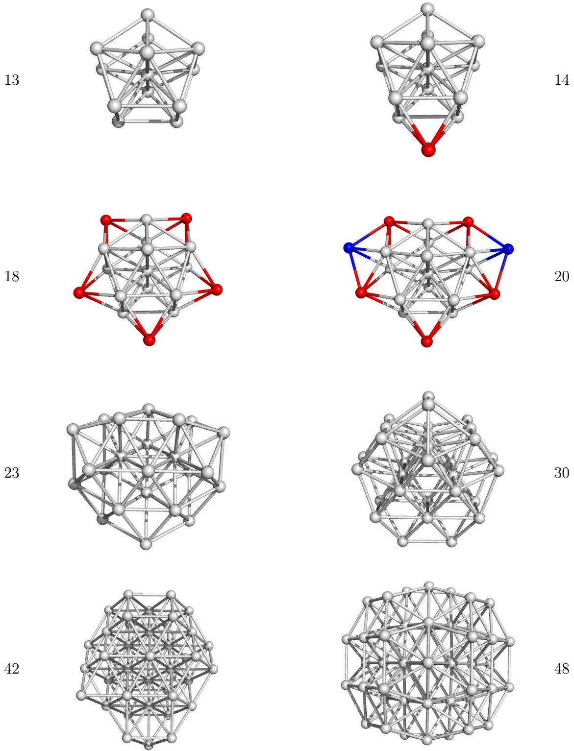
Figure 5.6: Clusters of particle interacting via the (\alpha = 18) -potential with 13, 14, 18, 20, 23, 30, 42 and 48 particles. Different colors indicate an observable growth pattern. See text for comments.
