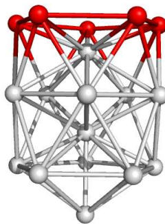
Figure 5.4: Growth pattern for Lennard-Jones clusters with N = 12 - 19 . Notice the variant structure at N = 17 .
