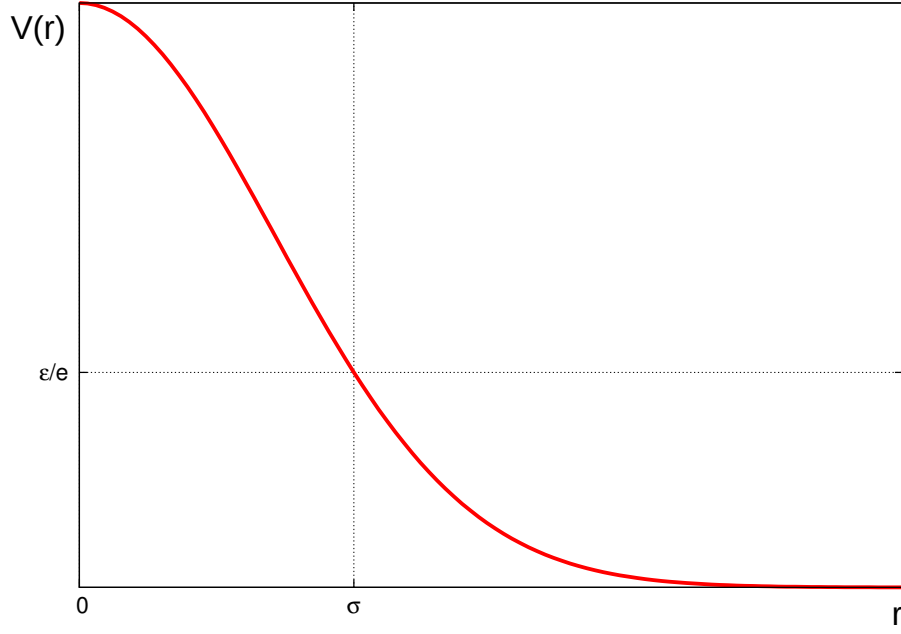
Figure 3.5: Gauss potential V_G(r) = \epsilon \exp \left( -\frac{r^2}{\sigma^2} \right) .
