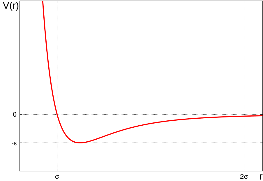
Figure 3.1: Lennard-Jones potential
