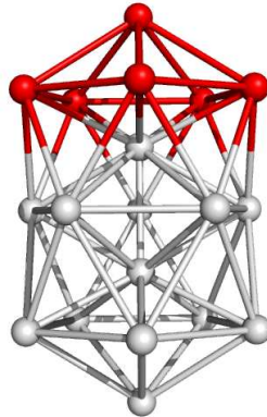
Figure 5.4: Growth pattern for Lennard-Jones clusters with N = 12 - 19 . Notice the variant structure at N = 17 .
