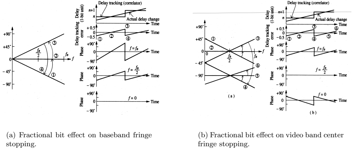
Figure 13: Implication of fringe stopping on fractional bits (Takahashi et al., 2000, [73]).
