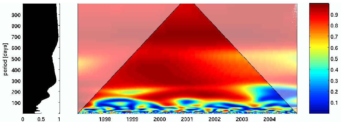
Figure 56: Quadratic cross-scalogram |W_{VLBI,GPS}(a,b)|^2 (right) and normalized Wavelet coherency (left) at station KOKEE.
