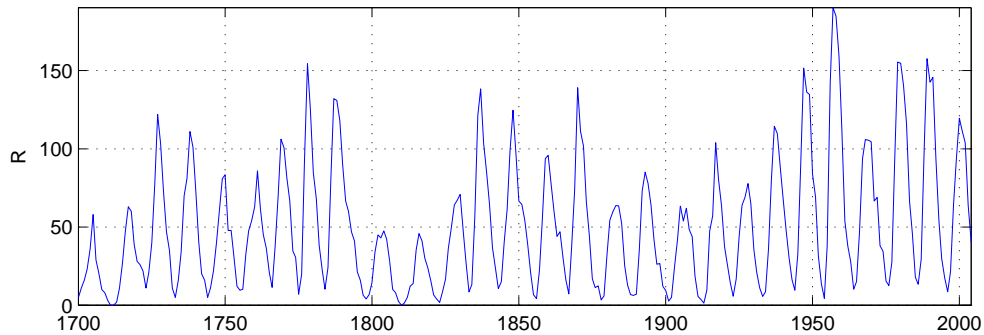
Figure 4: Plot of the annual sunspot numbers 1700-present (NGDC, 2005, [53]).
