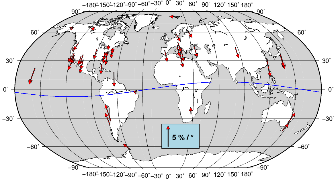
Figure 48: Global map of the averaged gradient-like parameters c_i .
