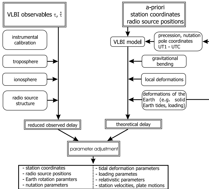
Figure 16: Flow diagram of geodetic VLBI data analysis.
