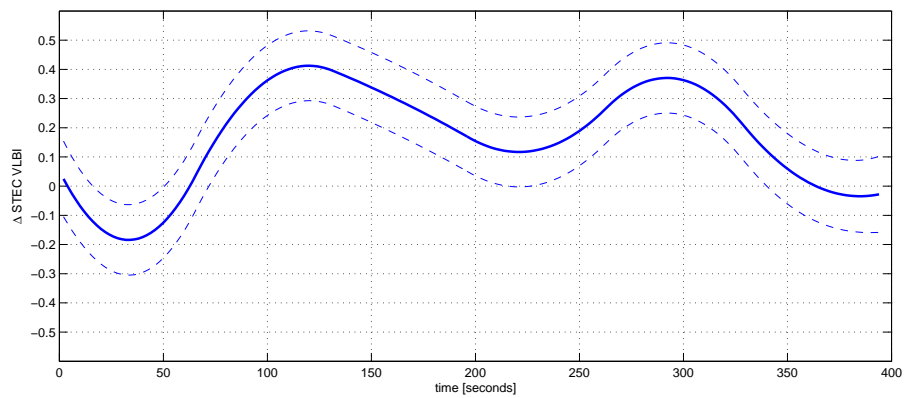
Figure 80: Intra-scan variation of \Delta\text{STEC} in TECU on Jan. 7th, 2004 from 8:48:00 UT until 8:54:50 on the baseline HARTRAO-HOBART26.
