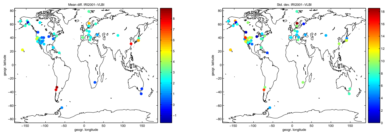
(a) Map of the mean differences between IRI2001 and VLBI.
