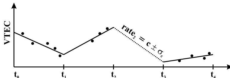
Figure 31: Equally spaced piece-wise linear function, constraints are needed for data gaps.
