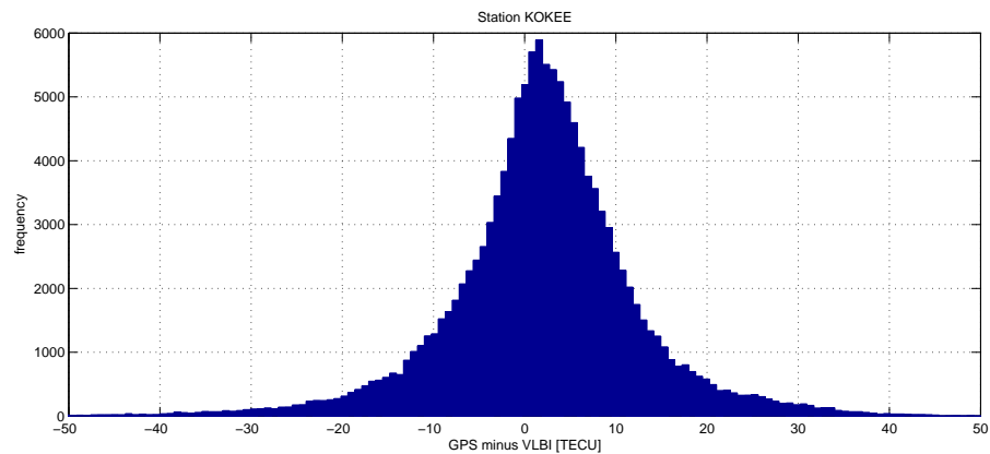
Figure 60: Differences of VTEC at station KOKEE between GPS and VLBI.
