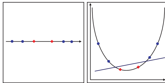
(a) not linearly separable (b) linearly separable
