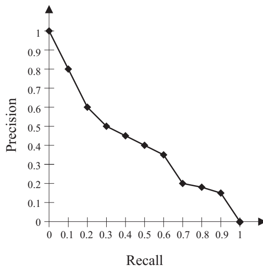
Figure 2: A typical Recall-Precision Graph, illustrating the tradeoff between Recall and Precision.
