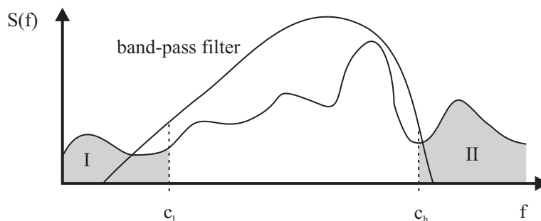
Figure 7: S(f) is the spectrum of a signal s(n) . The band-pass filter removes constant and slowly varying components below the low cut-off frequency c_l (area I). Furthermore, artifacts above the high cut-off frequency c_h are removed (area II).
