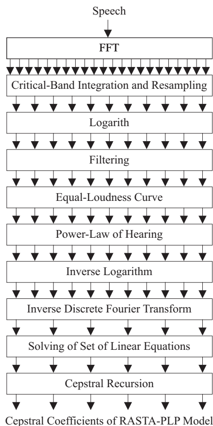
Figure 6: The RASTA-PLP method.
