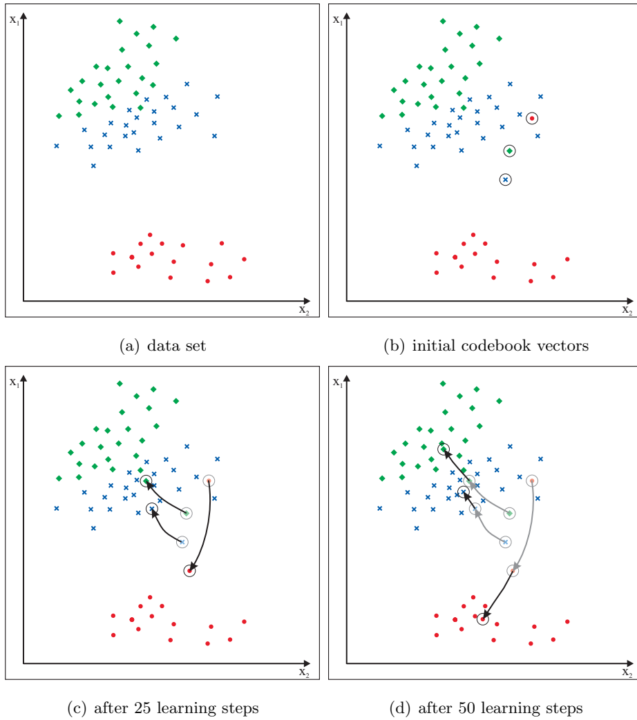
Figure 10: The learning process of the LVQ classifier: (a) the original data set with shape-coded class labels; (b) the circles mark the initial codebook vectors for each class; (c) and (d) display the path of the codebook vectors while they move towards the group of training patterns that belong to the same class.
