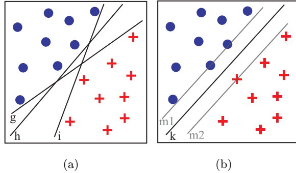
Figure 11: Optimal Separating Hyperplanes (OSH): (a) g, h, i are valid but not optimal separating hyperplanes. (b) k is the OSH, the distance between k and m1 respectively m2 is equal and maximal.
