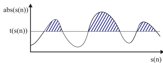
(c) AHA
