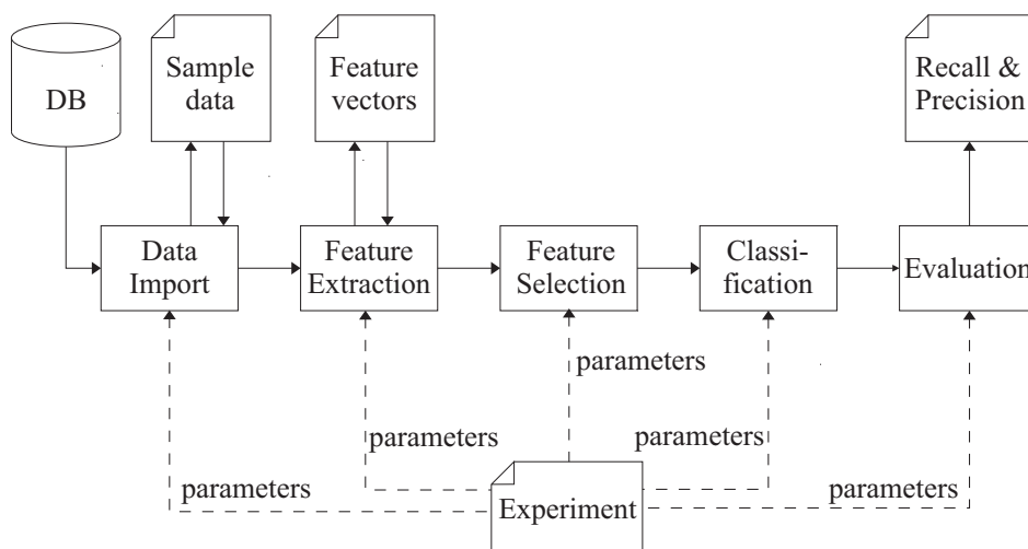
Figure 4: The MATLAB framework employed for the experiments. Each experiment is represented by a configuration file defining the parameters of the different retrieval processes, such as feature extraction, features selection, classification and evaluation.
