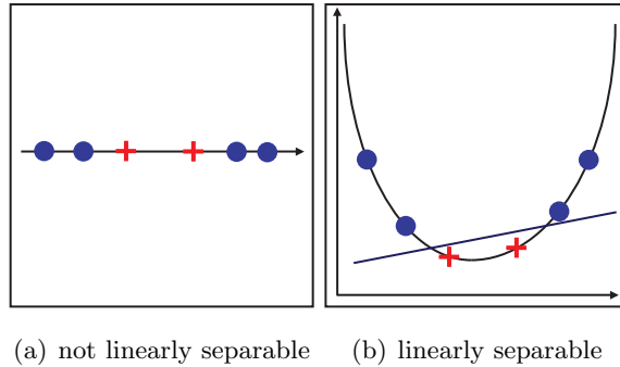
Figure 12: The kernel maps the one-dimensional input space (a) into a feature space of higher dimensionality, where the inputs become linearly separable (b).
