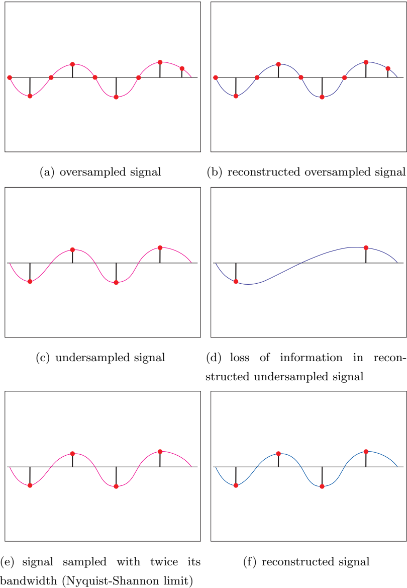
Figure 3: Audio sampling at different rates: 3(a) and 3(b) illustrate, that no gain is achieved by oversampling. The reconstructed signal in 3(b) is identical to the original signal. 3(c) and 3(d) show the devastating effect of undersampling. The signal cannot be reconstructed properly. Sampling at the optimal rate is depicted in 3(e) and 3(f).
