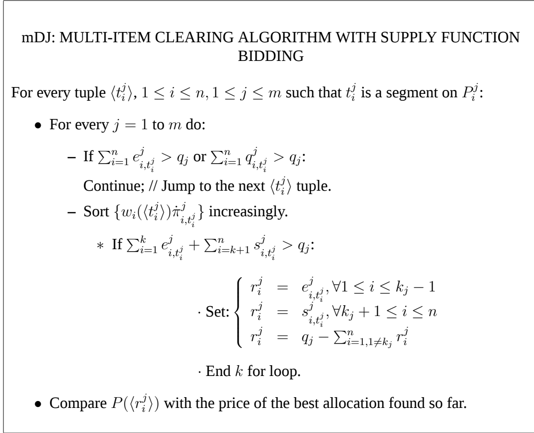
Figure 4.4: The mDJ clearing algorithm [DJ03] – Optimal clearing algorithm for multi item combinatorial auctions with supply function bidding.
