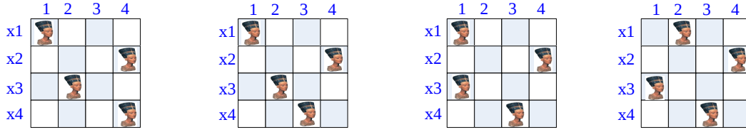
Figure 5.4: Execution example of the Asynchronous Weak-Commitment [YH00]
