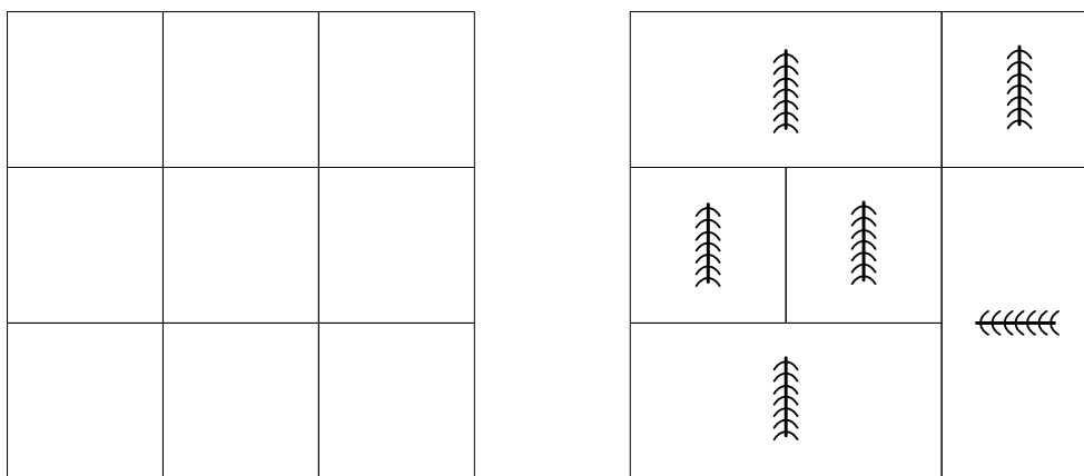
Figure 2.14: Plots of land to auction and possible result if bundles are permitted.
