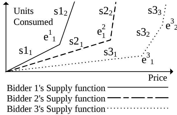
Figure 4.5: Linear piece-wise supply functions submitted to a single item – Each bid function is composed of a number of segments S_j^i , where i corresponds to the Bidder and j to the number of the segment, and end points e_k^j , where j shows the number of segments that ends there and k the number of end point.
