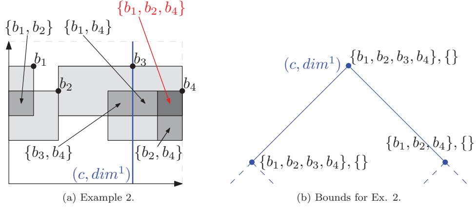
Figure 7.2: Illustration for example 2 depicting some domain crossing regions in 7.2a and corresponding segmentation tree in 7.2b.
