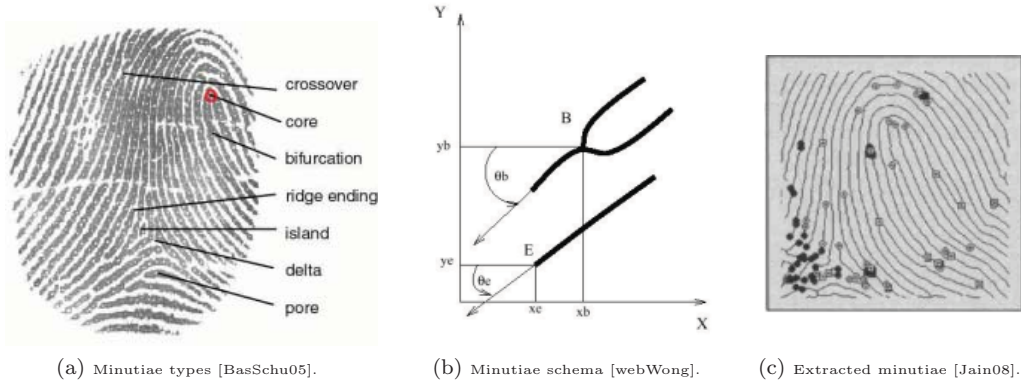
Figure 1.1: Fingerprint minutiae in dactyloscopy.
