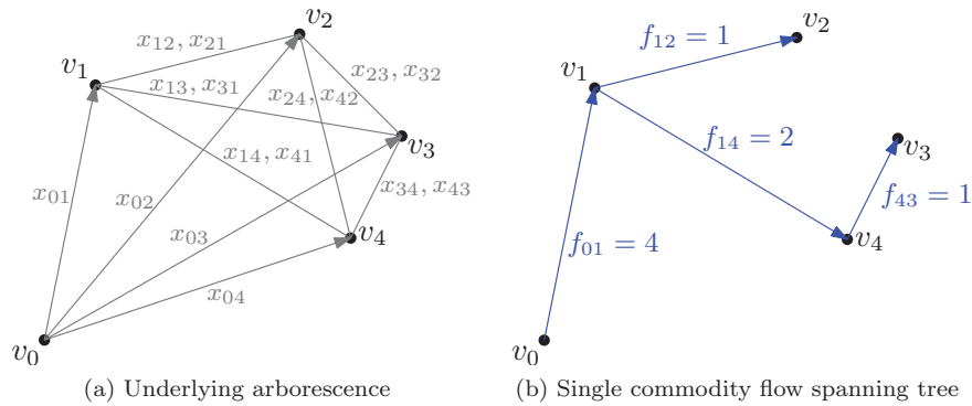
Figure 5.1: Single commodity flow network in an arborescence.
