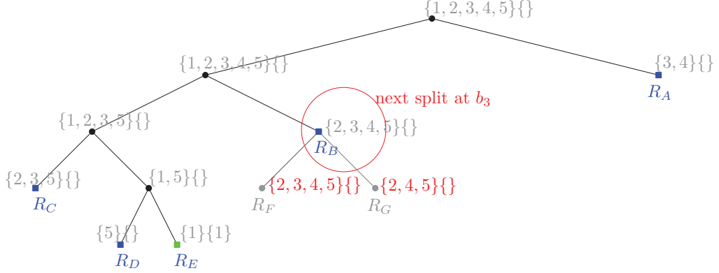
Figure 6.14: Dynamic segmentation tree resulting from 6.13b.
