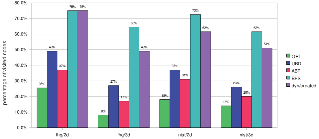
Figure 9.2: Averages percentage of visited nodes for the static UBD, ABT and BFS. Created nodes percentage (OPT) in a dynamic tree in relation to the minimal number of nodes for determining T^c , when visiting branches containing an element from T^c only once.
