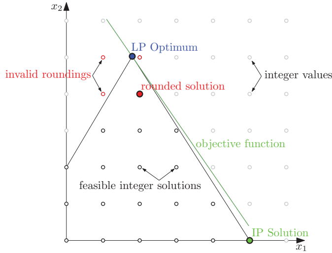
Figure 3.4: Rounding is not always a good idea in IP's and BIP's: The IP solution is far away from the rounded values. Image credits to [Wol98], page 4.
