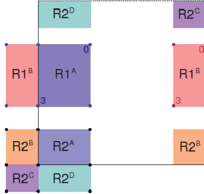
Figure 6.6: Partially negative regions and their transformation to the working domain. Regions R_{1A} and R_{2A} are regular, the other are modulo transformed into domain \mathbb{D} .
