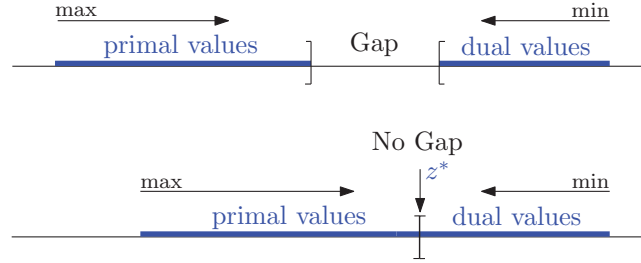
Figure 3.1: Duality Gap between largest primal and smallest dual value. Image credits to [Van98].
