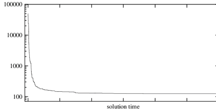
Figure 3.9: “The depicted development of the objective function value is typical for the tailing off effect.” Image credits to [Luebbe01].
