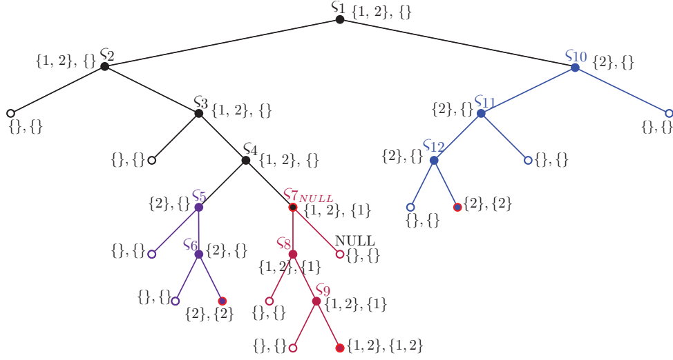
Figure 6.11: Segmentation tree with bounds after insertion of b_2 .
