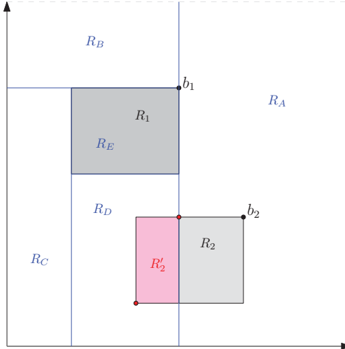
Figure 6.12: Rectangles show the regions that the node differences b_1 and b_2 define. If we arrive at node encoding subspace R_D and determine a part of R_2 to be inserted here, we crop the bounding box to the subspace by R'_2 = R_D \cap R_2 . The resulting R'_2 is marked by two red dots. At node containing R_D , we insert only this part R'_2 .
