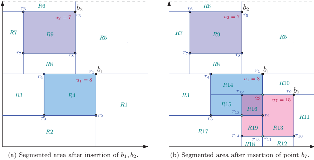
Figure 6.1: Segmentation of a sequence of points b_i . Figures 6.2 and 6.3 show the corresponding trees.
