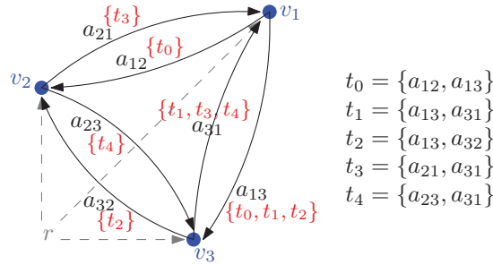
Figure 5.2: Correlation of tree arcs a and template arcs t (labels). When taking one of the template arcs t_0, t_2 or t_4 , we get a spanning tree, whereby t_1 forms a cycle and hence no spanning tree. Also t_3 forms no spanning tree.
