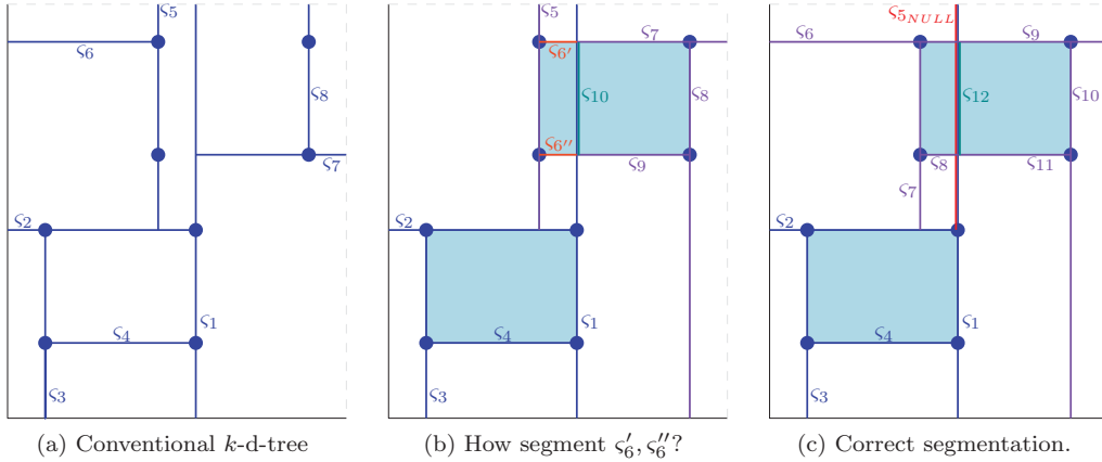
Figure 6.9: The reason, why null subspaces have to be inserted. How, in figure 6.9b, should s'_6, s''_6 be segmented and the dimension sequence retained? Figure 6.9c shows the correct segmentation by inserting a null subspace s_{5\_NULL} .
