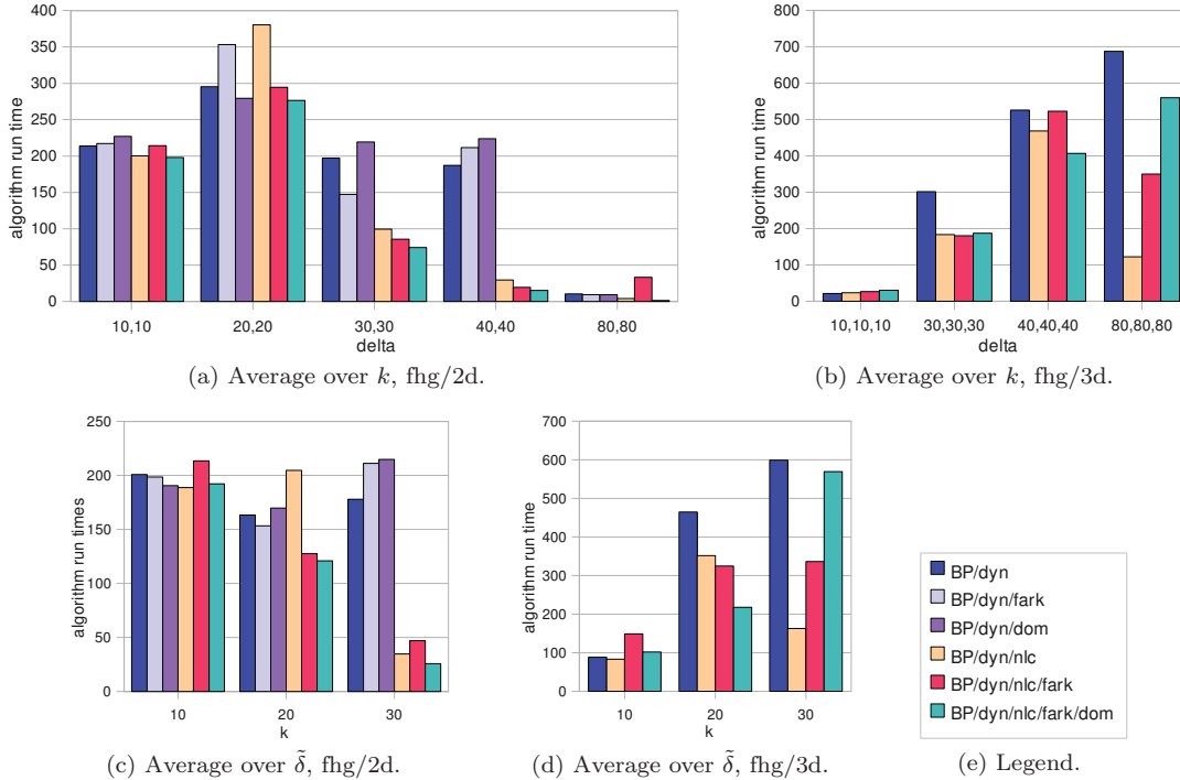
Figure 9.5: Performance of selected options for the dynamic tree pricing algorithm, figures 9.5a, 9.5b in the first row show the average over k , figures 9.5c, 9.5d in the second row the average over \tilde{\delta} .
