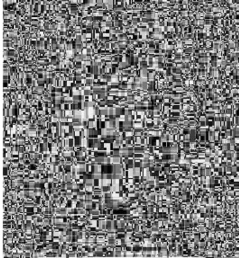
Black and white segmentation visualization, 2-d static tree, instance ft-03, \delta = (40, 40)^T
