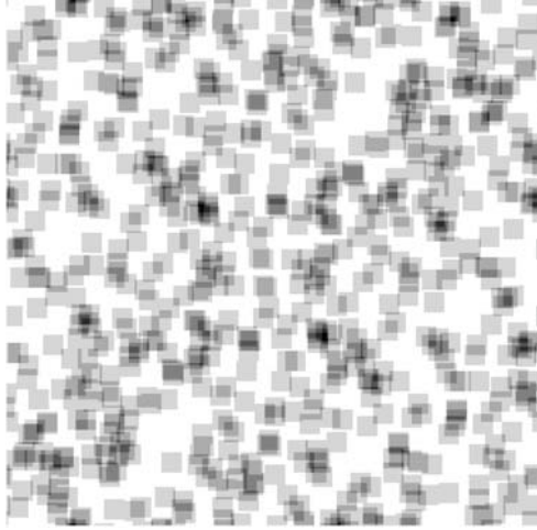
Visualization of bounding boxes, 2-d static segtree, instance ft-09, \delta = (10, 10)^T
