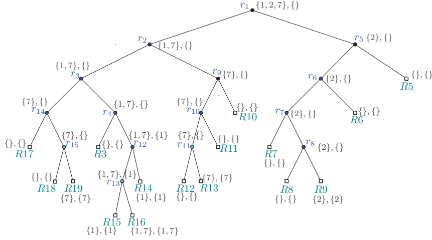
Figure 6.3: Segmentation tree after insertion of b_7 . A left son \cong left, below; right son \cong right, above.
