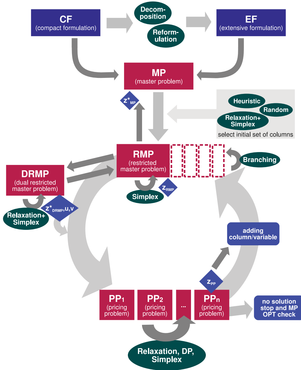
Figure 3.6: Column generation flowchart.
