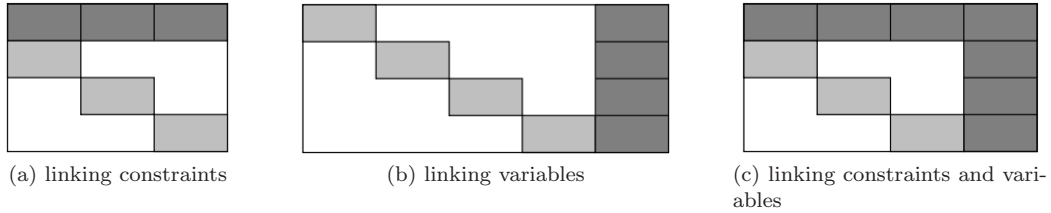
Figure 3.7: Example schemes of block diagonal matrices, shaded areas indicate nonzero elements [Luebbe01].
