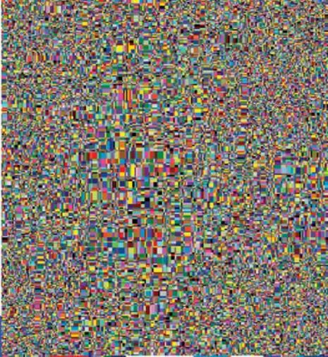
Color segmentation visualization, 2-d static tree, instance ft-03, \tilde{\delta} = (40, 40)^\top
