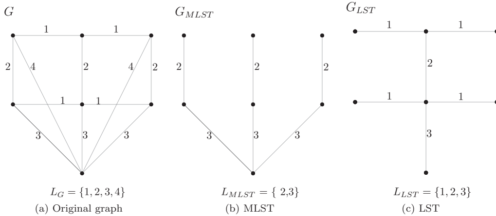
Figure 2.1: Figure 2.1b shows an optimal MLST, determined from the labeled graph in figure 2.1a. Figure 2.1c is a possible Label Spanning Tree (LST) . Images adopted from [XiGolWas05].
