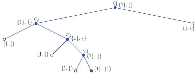
Figure 6.8: Segmentation tree after insertion of b_1 .
