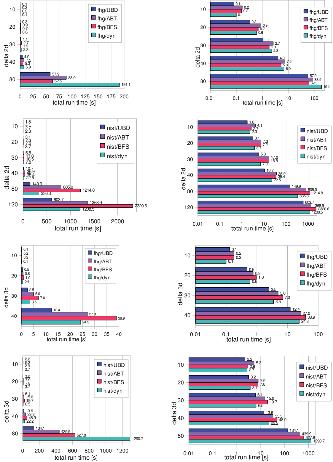
Figure 9.3: Fhg, nist instances running times for each traversing strategy, including the dynamic tree for 2- and 3-dimensional \tilde{\delta} . On the left side we used a linear scale, on the right side a logarithmic scale in order to make visible the differences for run times with small \tilde{\delta} .
