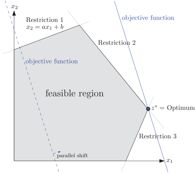
Figure 3.2: Example of a geometric interpretation.
