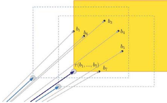
Figure 4.1: “The big gray dots are three of the possible representants for the tree arcs b_1, \dots, b_7 , but the standard template arc \tau is the lower left point of the shaded rectangle. The rectangles depict the \tilde{\delta} domain.” Image credits to [ChwRai09].
