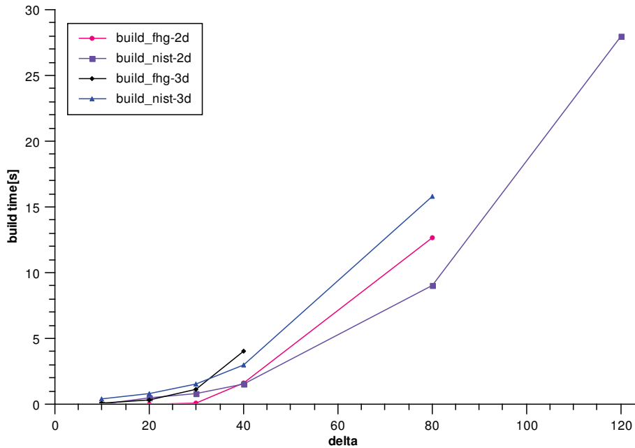
Figure 9.1: Growth rates of static tree building time, distinguished by dimensionality of \tilde{\delta} as well as by data set (fhg and nist).
