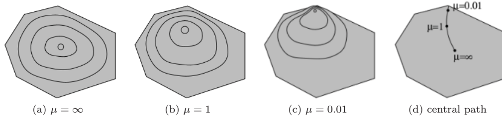
Figure 3.3: Figures 3.3a - 3.3c show contour lines of a logarithmic barrier function for three values for the pace parameter \mu . The maximum value lies inside the innermost level set. Figure 3.3d depicts the central path . Image credits to [Van98].
