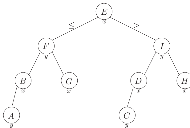
Figure 2.3: Balanced 2-d tree resulting from the construction steps in figure 2.2.
