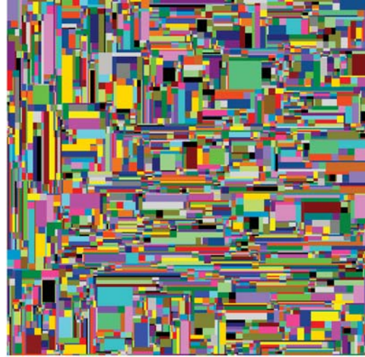
Color segmentation visualization, 2-d static tree, instance ft-09, \delta = (5, 5)^T
