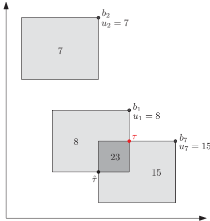
Figure 6.4: A standard template arc \tau for the segmentation in figure 6.1b.
