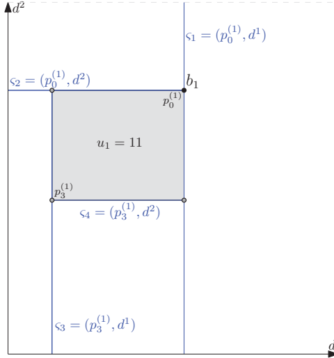
Figure 6.7: Simple segmentation of node difference b_1 . The figure shows four splits \varsigma , two at p_0^{(1)} and two at p_{2^d-1}^{(1)} . The resulting segmentation tree is depicted in figure 6.8.
