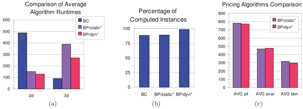
Figure 9.6: Average run times, completed instances, pricing data for ‘BC’ and the best branch-and-price variants ‘BP/static/nlc/fark’ (abbreviated by ‘BP/static*’) and ‘BP/dyn/nlc/fark’ (abbreviated by ‘BP/dyn*’). Run time averages over \tilde{\delta} , k .
