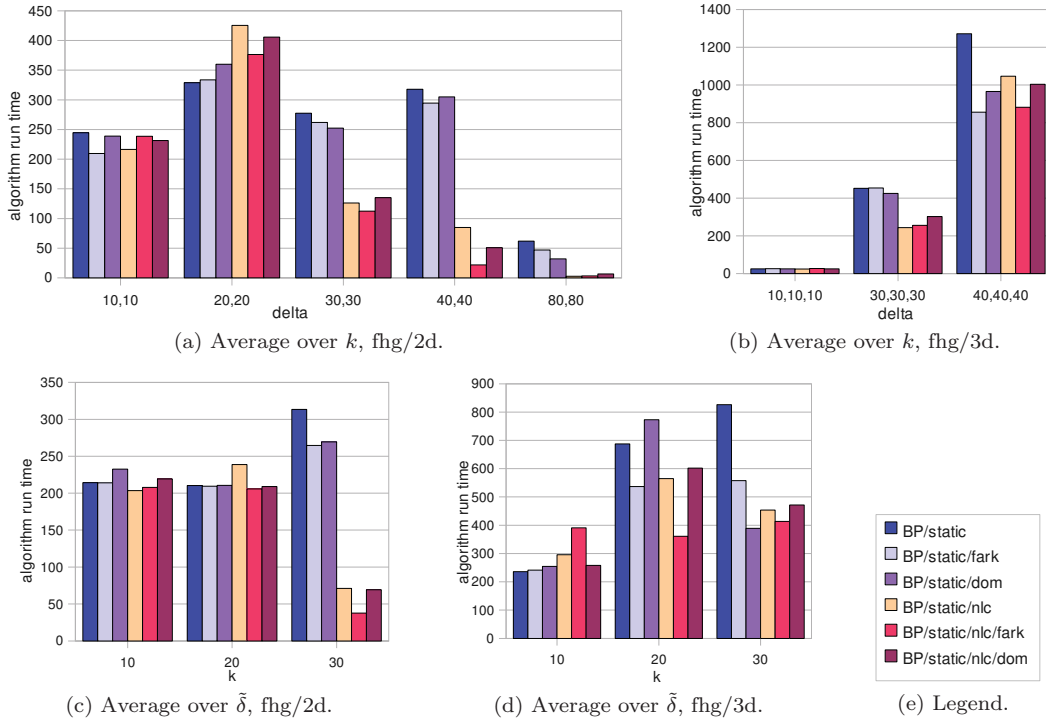
Figure 9.4: Performance of selected options for the static tree pricing algorithm, figures 9.4a, 9.4b in the first row show the average over k , figures 9.4c, 9.4d in the second row the average over \tilde{\delta} .
