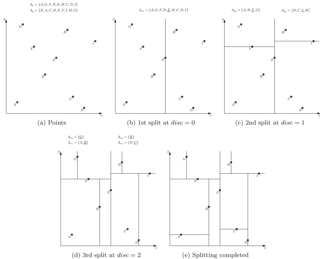
Figure 2.2: Construction of a balanced 2-d tree. The rounding median depends on the implementation. Here the median is round-up.
