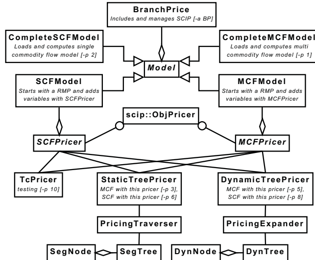
Figure 8.2: Class diagram for the parts concerning branch-and-price.
