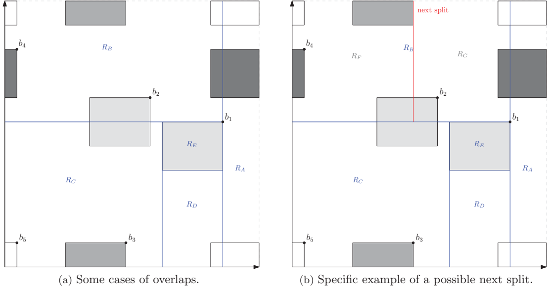
Figure 6.13: Some cases of overlaps. In figure 6.13a, the case for b_4 is interesting since it reaches into the node subspace R_2 again across the domain border. Parts of subspace b_5 reach into even more node subspaces. When having big \tilde{\delta} such overlaps occur very often. All other cases are trivial. Figure 6.13b shows a specific example of a possible next split. The figure shows the segmentation after insertion of b_1 . The region for b_3 will be inserted next. The next split is drawn in red.
