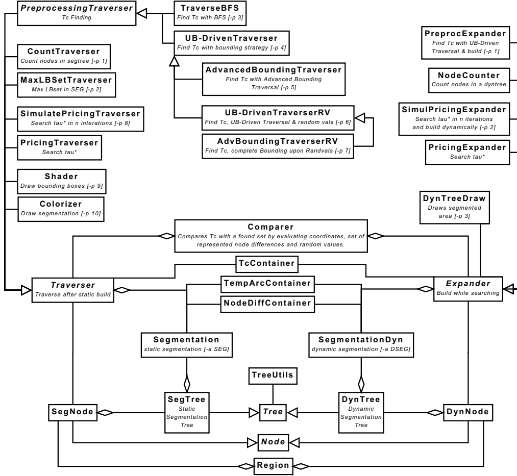
Figure 8.1: Class diagram for the parts concerning segmentation and traversing.
