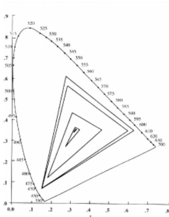
Figure 3.5: Chromatic gamut of CRT for ambient illumination covering a range of five log units. [Layc83]
