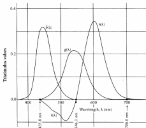
Figure 2.2: The r , g , and b color-matching curves [WySt82]
