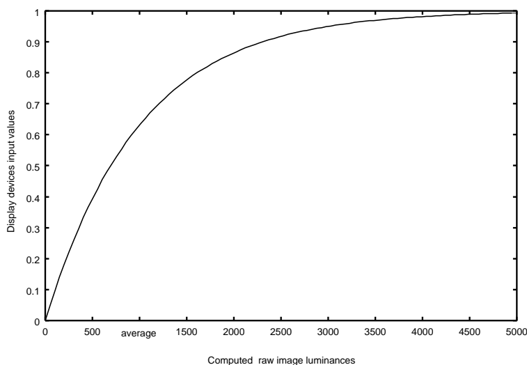
Figure 5.1: Exponential mapping
