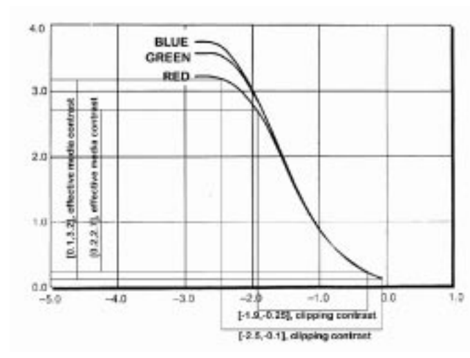
Figure 3.3: The characteristic curves of Kodak Ektachrome Panther 100x Professional
