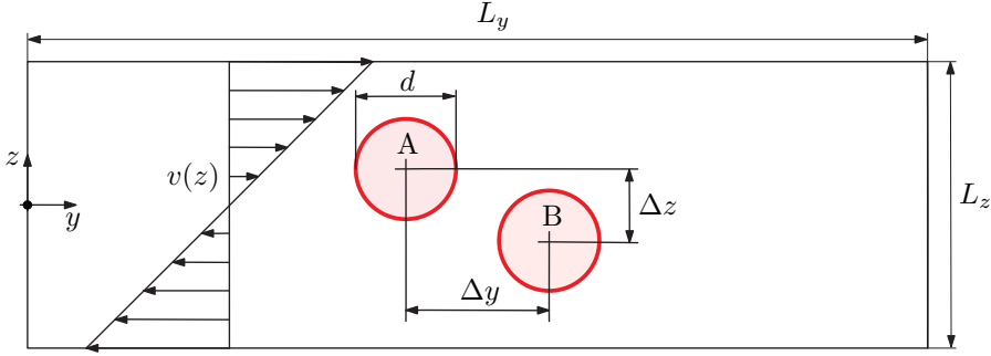
FIGURE 5.1 – Simulation setup used to analyze the effects of a dissolved surfactant on binary droplets interactions. Two circular droplets, d = 0.7 , are placed at y_c = \pi \mp 0.5 and z_c = \pm 0.25 (coordinates of the droplets center of mass at the beginning of the simulation). The offset in the streamwise direction is \Delta y = 1 , while in the wall-normal direction is \Delta z = 0.5 . The two walls move in opposite directions, generating a laminar shear flow in the channel, v(z) .
