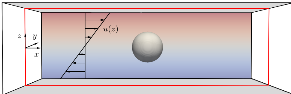
FIGURE 4.1 – Sketch of the computational domain used to analyze the deformation of a single droplet in shear flow. The domain has dimensions L_x \times L_y \times L_z = 2\pi h \times \pi h \times 2h for the 3D simulations and L_x \times L_z = 2\pi h \times 2h for the 2D simulations (red rectangle). A spherical droplet (circular for the 2D simulations) is initialized in the centre of the channel ( x_c = \pi h , y_c = \pi h/2 , z_c = 0 ). The two walls, located at z = \pm h and represented in grey, move in opposite directions with constant velocity u = \pm u_w .
