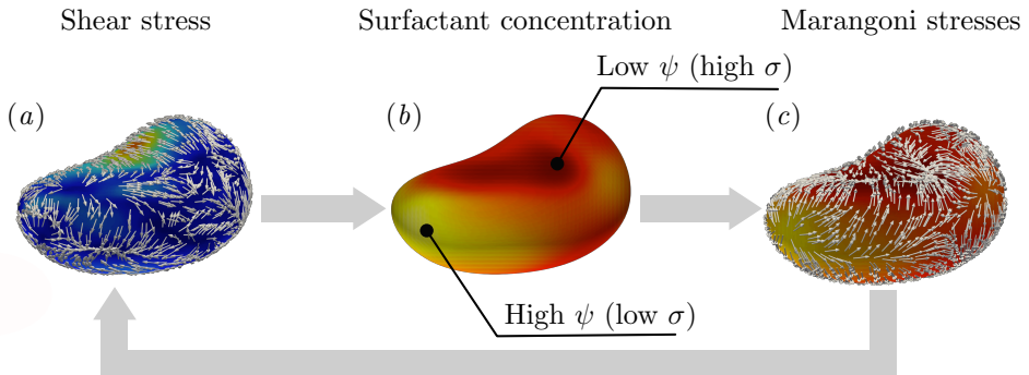
FIGURE 6.5 – Sketch of the coupling between shear and Marangoni stresses. The sketch is realized considering the droplet marked by the yellow box in figure 6.3(d). Panel (a) shows the component tangential to the interface of the shear stresses, \mathbf{S}_t , on the droplet interface and normalized by its magnitude. The interface is colored by the shear stress magnitude (blue–small; red–large). Panel (b) shows the resulting non-uniform surfactant distribution (red–low; yellow–high). This distribution, in turn, leads to a non-uniform surface tension distribution and thus gives rise to Marangoni stresses, shown in panel (c) using unit length vectors. These stresses try to restore a uniform value of the surface tension driving flow from high surfactant concentration regions (yellow) towards regions with a lower concentration (red). Marangoni stresses feeds back onto the local shear stresses distribution (right to left arrow).
