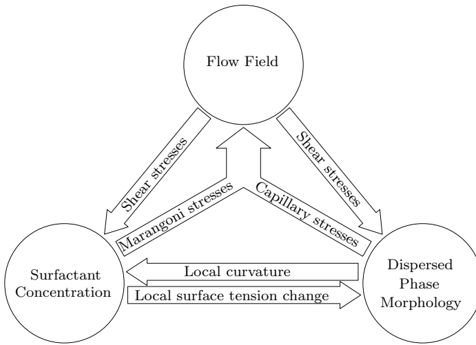
FIGURE 6.4 – Graphic representation of the main interactions among flow field, dispersed phase morphology and surfactant concentration. On one hand, the shear stresses produced by the flow field affect the dispersed phase morphology and the surfactant distribution (top to bottom arrows). On the other hand, capillary and Marangoni stresses influence the local flow field (bottom to top arrows). Then, also the dispersed phase morphology and the surfactant concentration mutually interact: the surfactant distribution locally reduces surface tension and increases the interface deformability (left to right to arrow). This effect is reflected in the interface morphology and dynamics, which in turn affect the surfactant distribution (right to left arrow).
