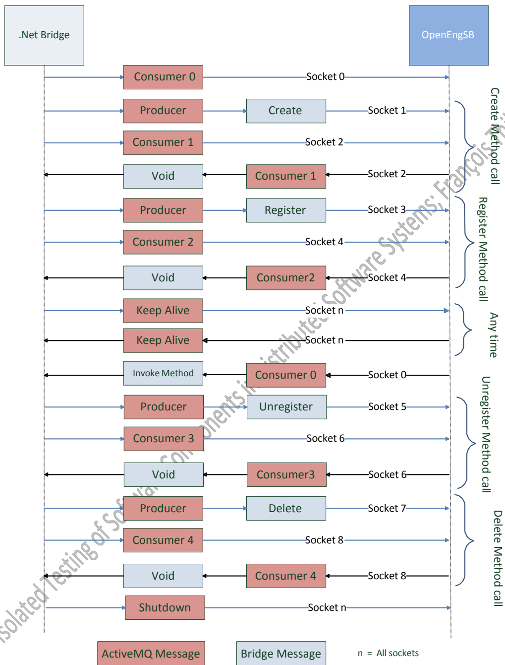
Figure 6.23: ActiveMQ and .Net Bridge communication
