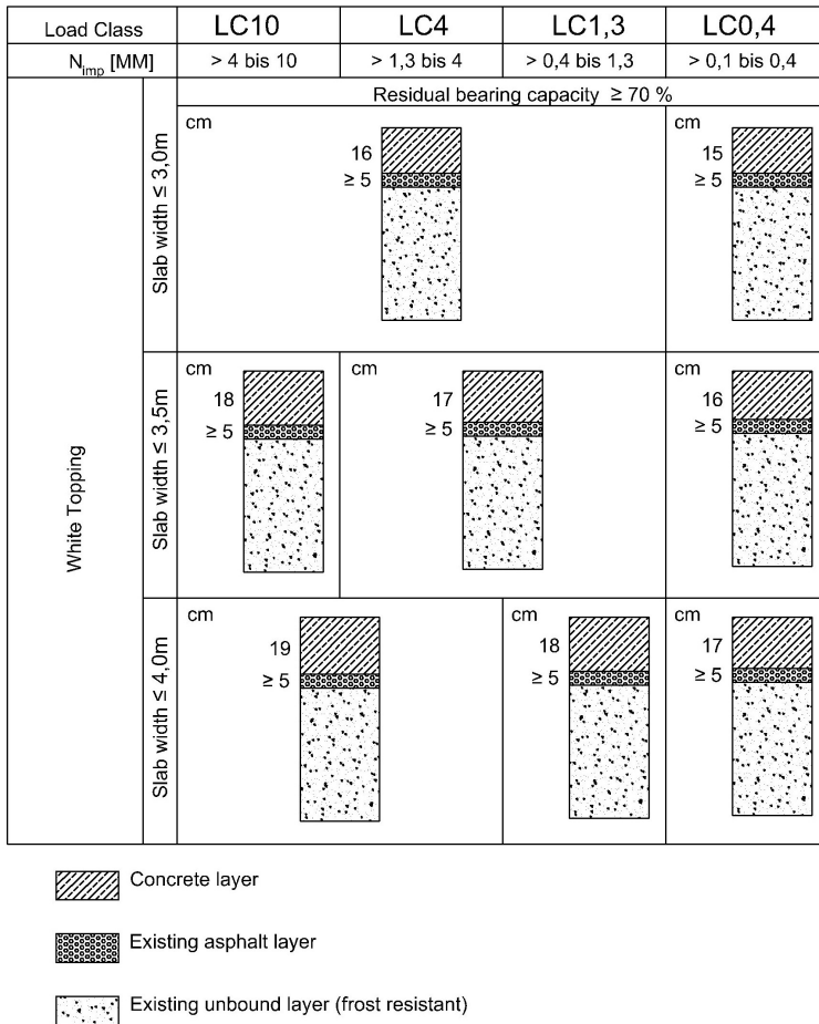
Figure 2. Developed Design catalog for bonded whitetopping pavements
