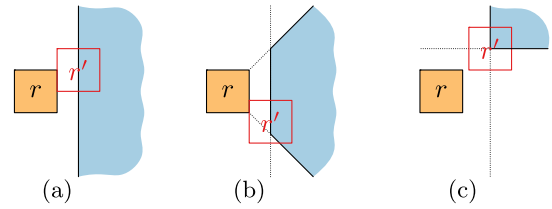
Fig. 4. Feasibility area (in blue) where r' may be placed w.r.t r , when r' is primarily to the right of r . (a) Our weak setting and the weak order constraints in [26] coincide. (b) The (“orthogonal”) order constraint in [26]. (c) Feasibility in our strong setting.
