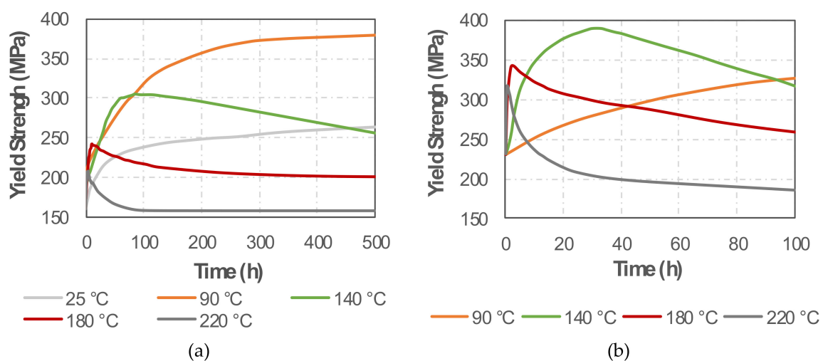
Figure 9. Simulated yield strength for various ageing treatments at various temperatures of: (a) single-stage treatment; (b) second treatment of double-stage treatment after ageing at 90 °C for 24 h.
