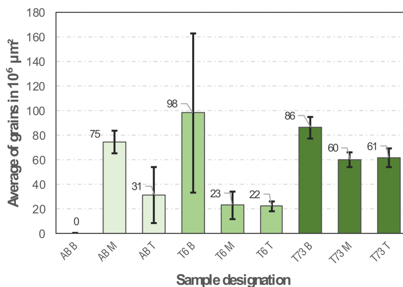
Figure 8. Average of grains in 10 6 μm 2 of the samples in the AB, T6 and T73 conditions.
