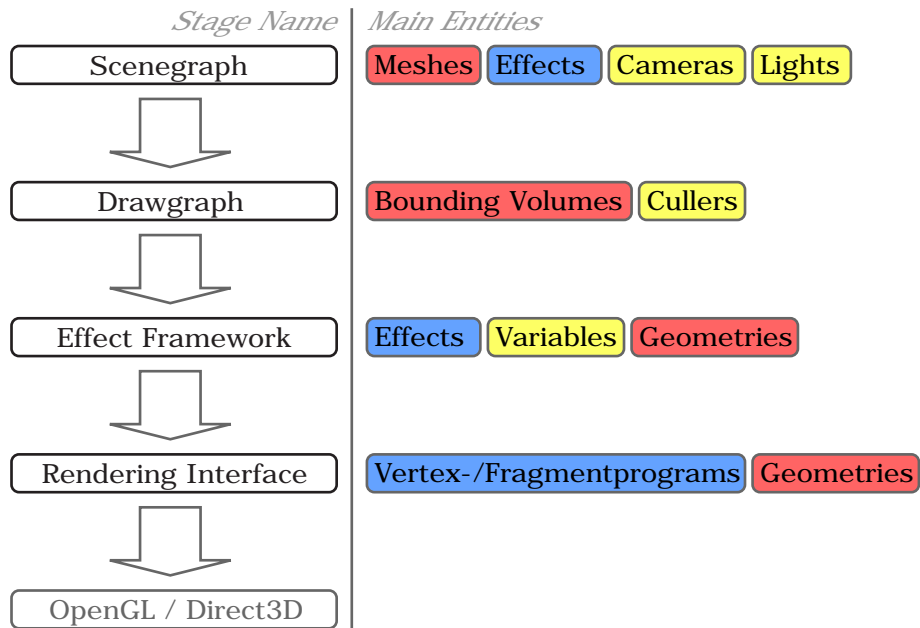
Figure 3.3: The graphics pipeline of YARE
