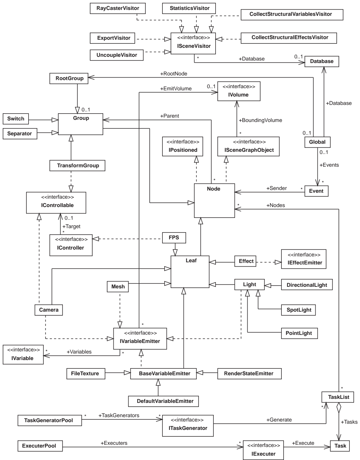
Figure B.2: The UML diagram of the scenegraph
