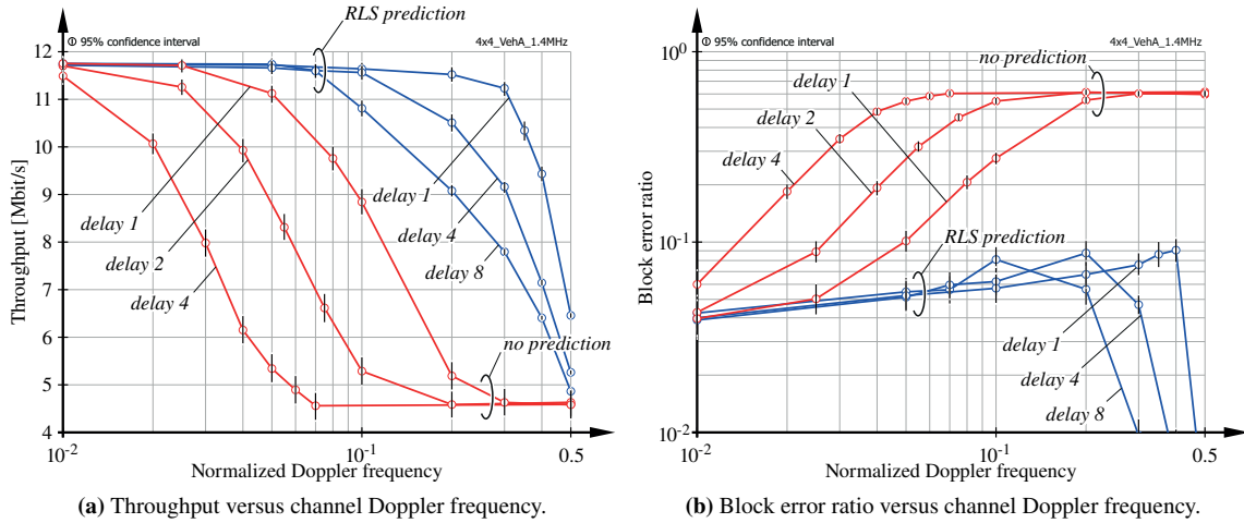
Figure 3.7.: Sensitivity of the proposed instantaneous CSI feedback algorithms with respect to a delay in the feedback path.
