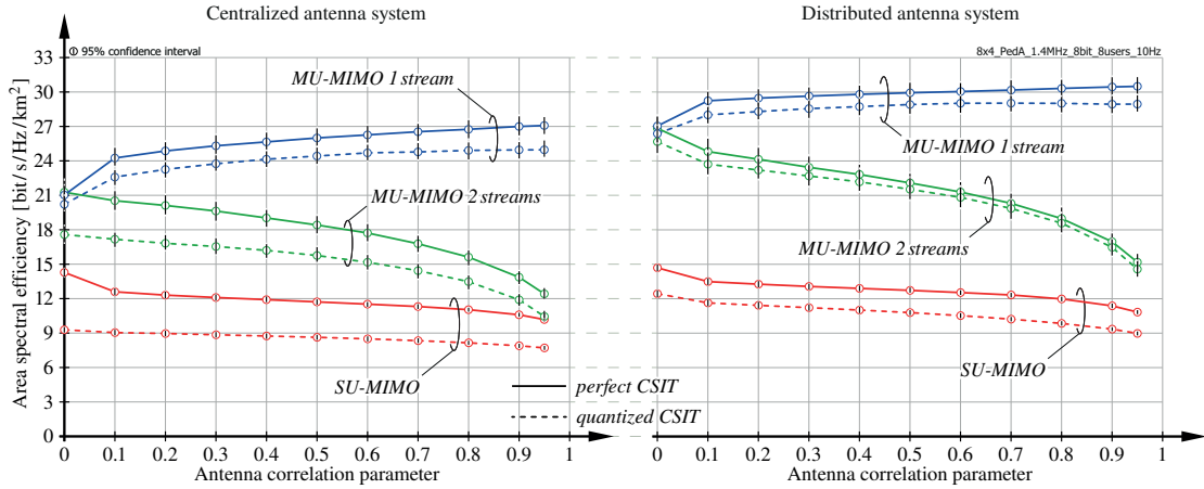
Figure 5.3.: Area spectral efficiency achieved in the CAS and the DAS in dependence of the receive antenna correlation. An N_i \times M_{u,i} = 8 \times 4 antenna configuration is considered, serving U_i = 8 user over \ell_{u,i} \in \{1, 2\} streams per user in case of MU-MIMO, and over up to \ell_{u,i} = 4 streams in case of SU-MIMO.
