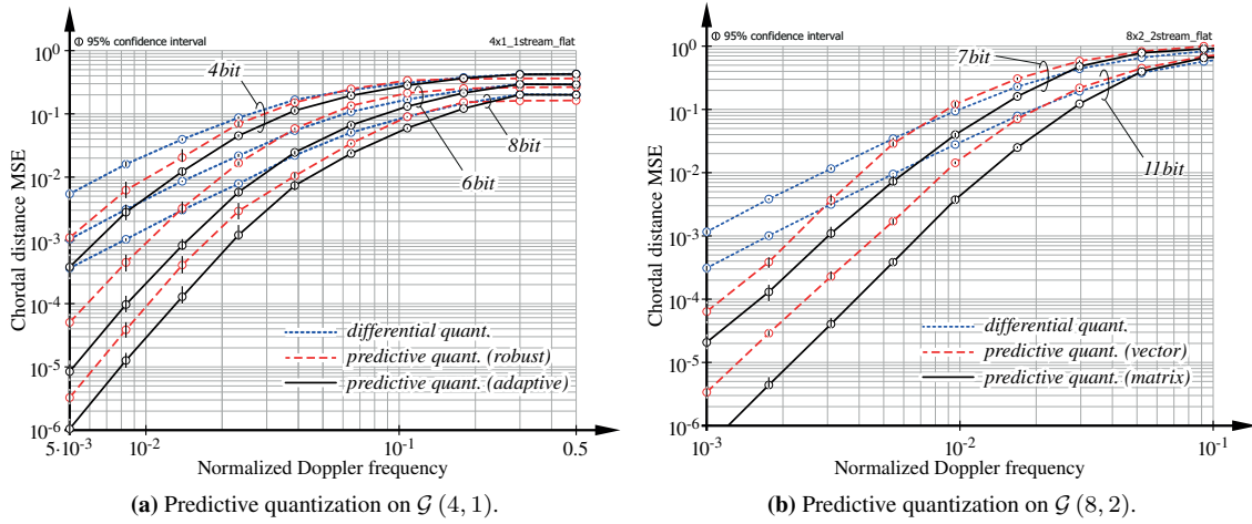
Figure 4.2.: MSE performance comparison of the proposed predictive Grassmannian quantizer using different prediction algorithms.
