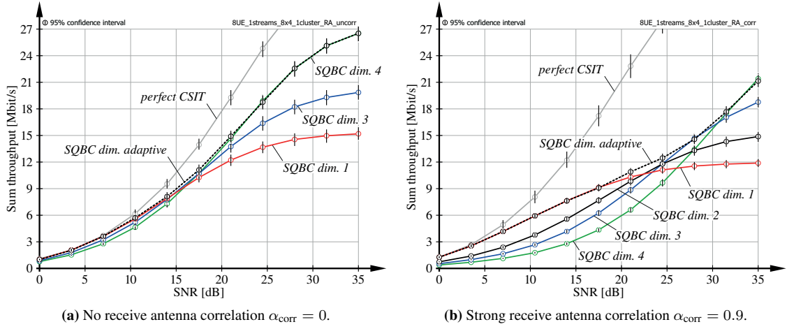
Figure 4.7.: Sum throughput achieved with ZF beamforming and SQBC feedback clustering in an N_i \times M_{u,i} = 8 \times 4 system, serving S_i = 8 users over \ell_{u,i} = 1 spatial stream each. The impact of dimensionality adaptation is investigated.
