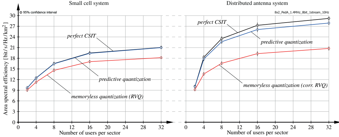
Figure 5.6.: Area spectral efficiency achieved in the DAS and the small cell system in dependence of the number of users per sector. An N_i \times M_{u,i} = 8 \times 2 antenna configuration is considered, transmitting \ell_{u,i} = 1 stream per user employing ZF based MU-MIMO.
