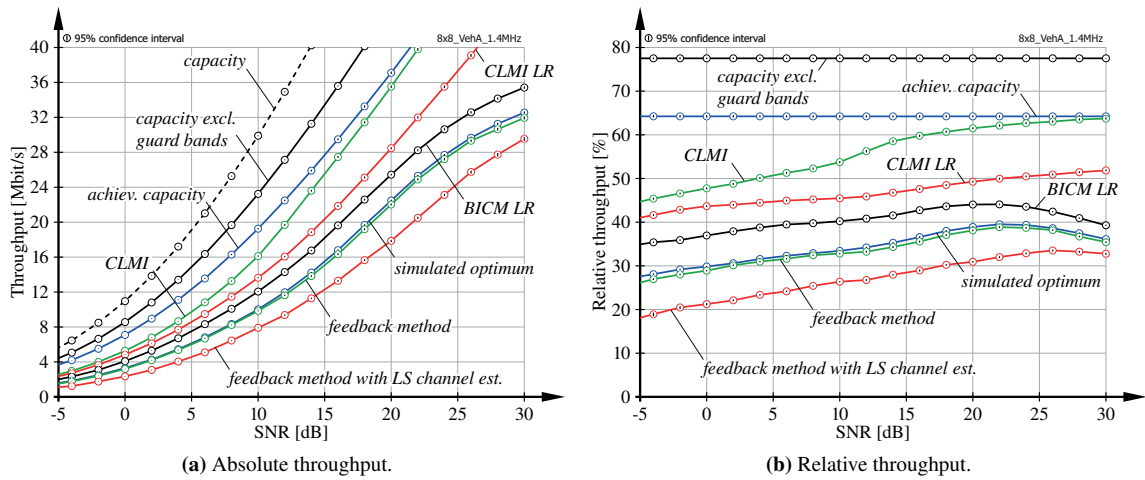
Figure 3.4.: Comparison of the achieved throughput to channel capacity and the proposed throughput bounds with N_i \times M_{u,i} = 8 \times 8 .
