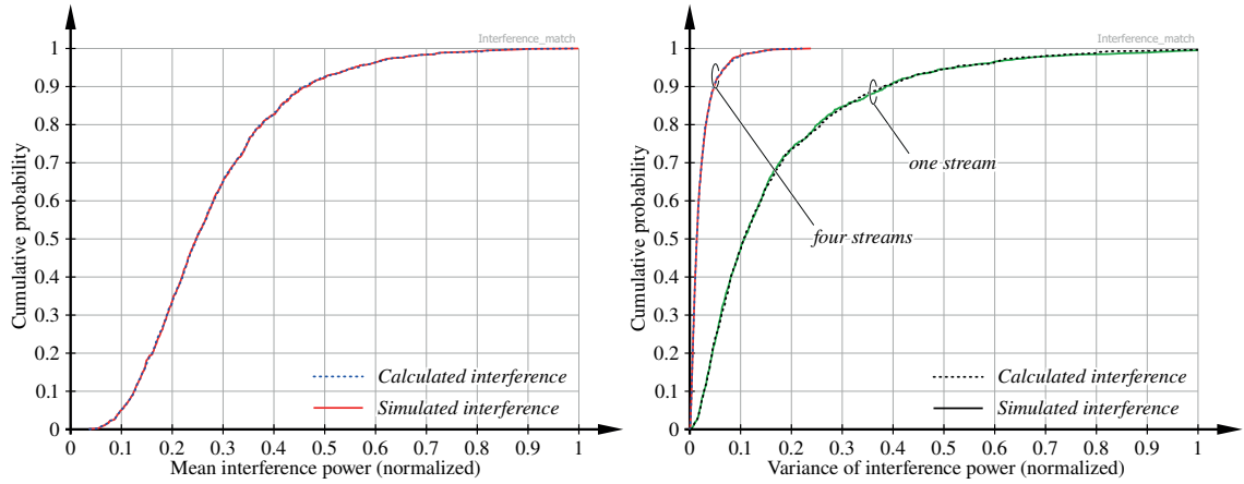
Figure I.1.: Cumulative probability of the mean and variance of the out-of-cell interference power of a single interferer receiving one or four spatially multiplexed data streams.
