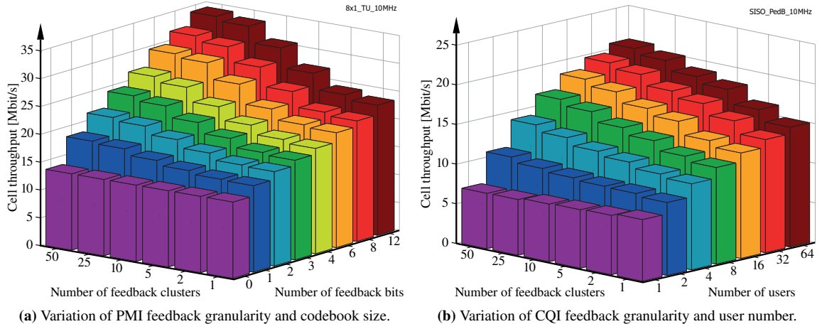
Figure 3.8.: Cell throughput with proportional fair scheduling versus CSI feedback granularity, codebook size and number of users.
