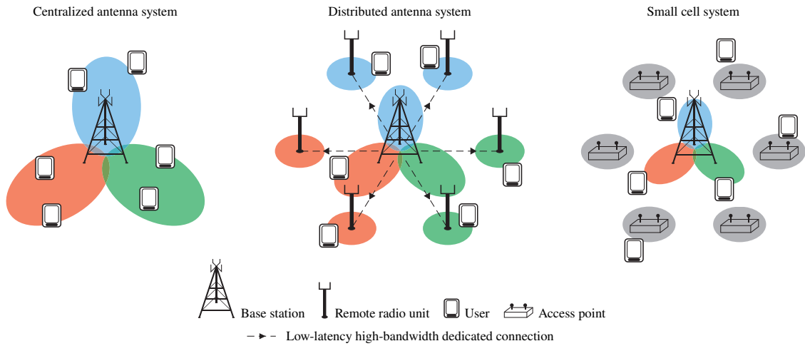
Figure 5.1.: Investigated cellular networking architectures.
