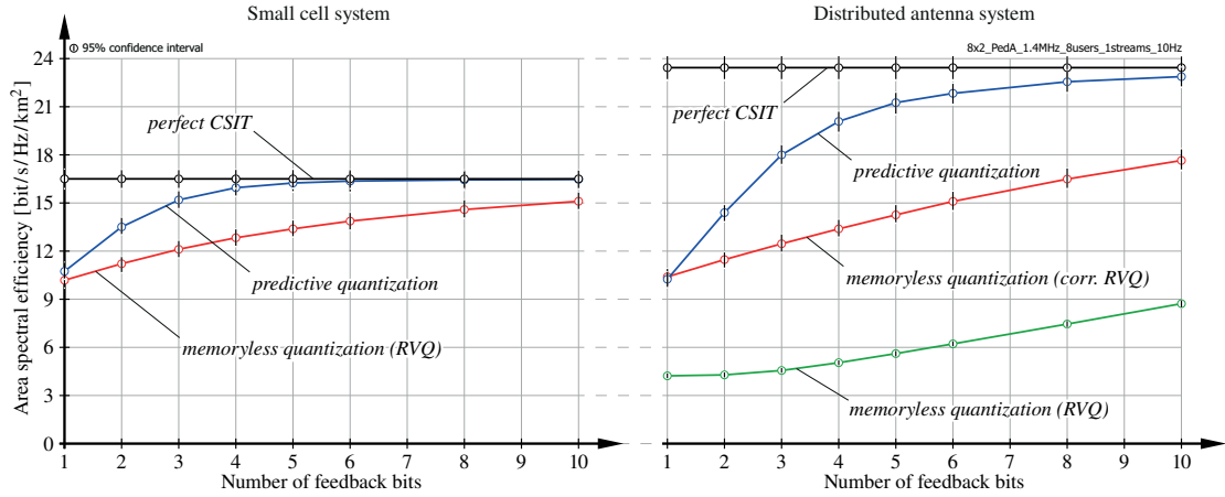
Figure 5.7.: Area spectral efficiency achieved in the DAS and the small cell system in dependence of the feedback overhead. An N_i \times M_{u,i} = 8 \times 2 antenna configuration is considered, serving U_i = 8 user over \ell_{u,i} = 1 stream per user employing ZF based MU-MIMO.
