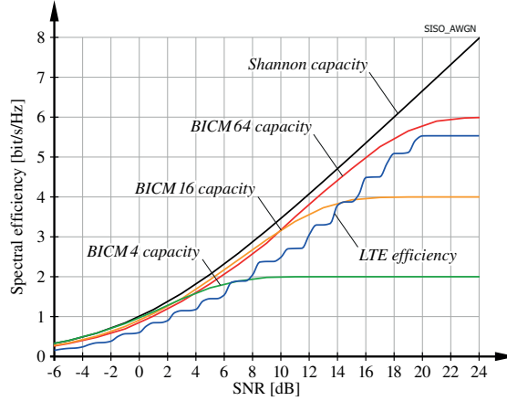
Figure 3.2.: Shannon capacity versus BICM capacity and the efficiency of LTE over an AWGN channel.
