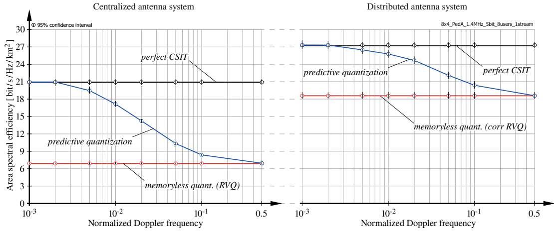
Figure 5.5.: Area spectral efficiency achieved in the CAS and the DAS in dependence of the channel Doppler frequency. An N_i \times M_{u,i} = 8 \times 4 antenna configuration is considered, serving U_i = 8 user over \ell_{u,i} = 1 stream per user employing ZF based MU-MIMO.
