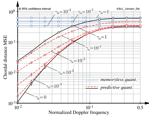
Figure 4.3.: Quantization MSE achieved with memoryless and predictive quantization in a DAS with varying channel gain differences.
