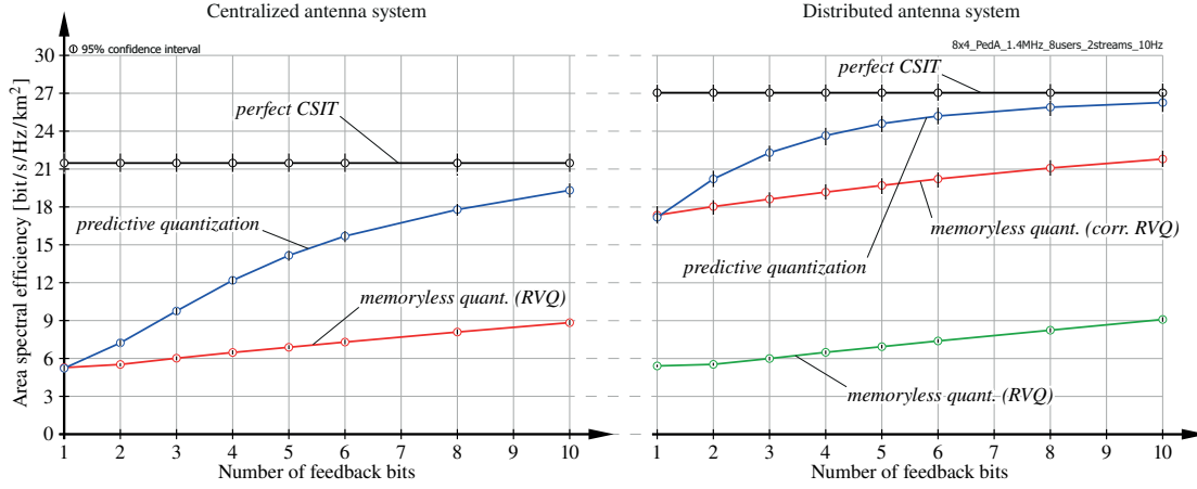
Figure 5.4.: Area spectral efficiency achieved in the CAS and the DAS in dependence of the feedback overhead. An N_i \times M_{u,i} = 8 \times 4 antenna configuration is considered, serving U_i = 8 user over \ell_{u,i} = 2 streams per user employing BD based MU-MIMO.
