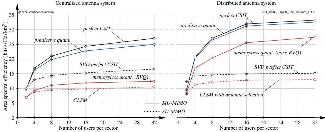
Figure 5.2.: Area spectral efficiency achieved in the CAS and the DAS in dependence of the number of users per sector. An N_i \times M_{u,i} = 8 \times 4 antenna configuration is considered, transmitting a single stream per user, \ell_{u,i} = 1 , to at most eight users in parallel in case of MU-MIMO, and up to \ell_{u,i} = 4 streams with SU-MIMO.
