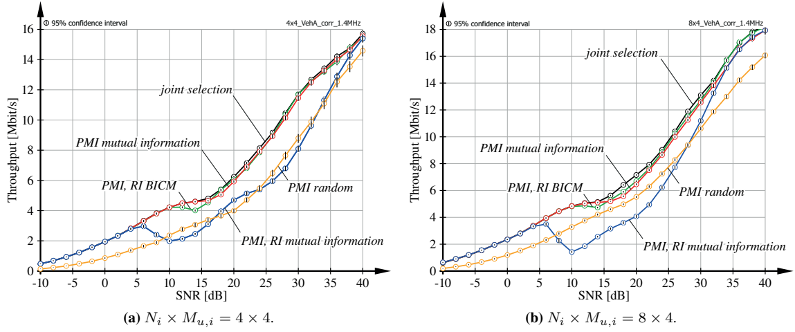
Figure 3.6.: Performance of approximate sequential CSI feedback selection schemes compared to the joint optimization.
