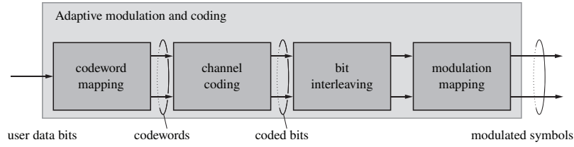
Figure 3.1.: AMC based on a BICM architecture according to the LTE specifications.
