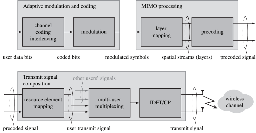
Figure 2.2.: MIMO OFDM transceiver architecture as considered in this dissertation.
