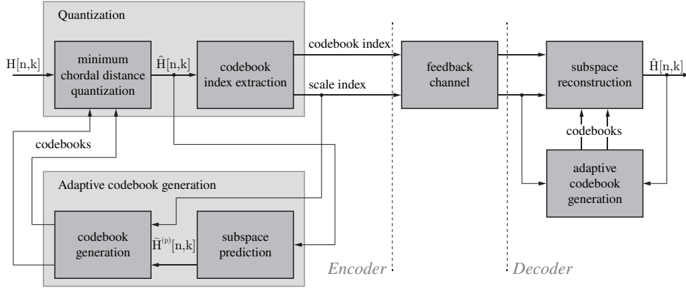
Figure 4.1.: Structure of the Grassmannian subspace quantizer visualizing the different components.
