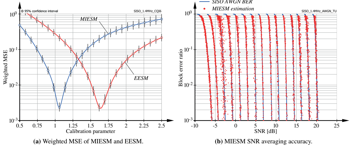
Figure E.1.: Calibration of effective SNR mapping and comparison of the MIESM abstraction for a 1.4 MHz typical urban channel to the average BLERs of the 15 LTE defined MCSs achieved over a 1.4 MHz AWGN channel.
