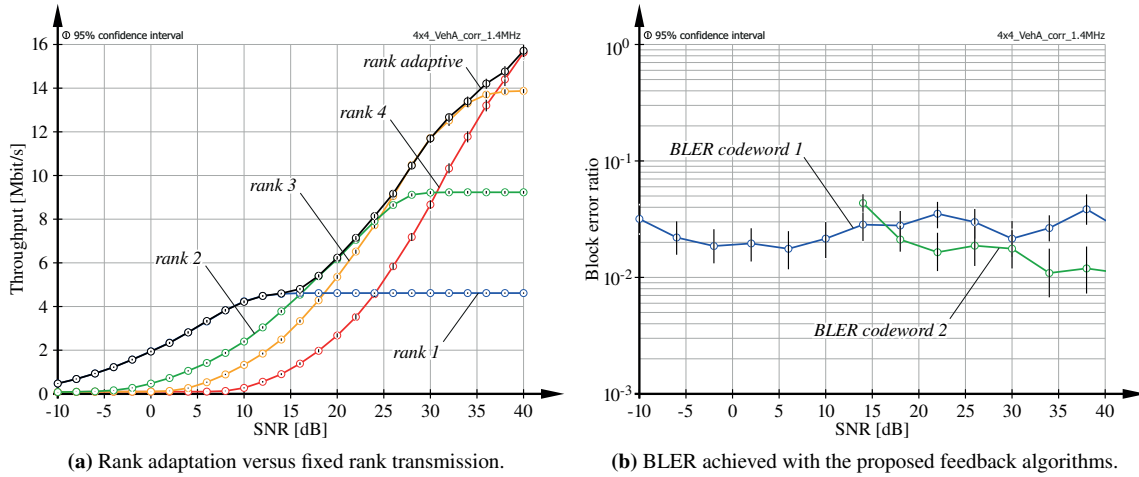
Figure 3.5: Comparison of the proposed rank adaptive scheme to fixed rank transmission and simulated BLER achieved with the proposed feedback algorithms.
