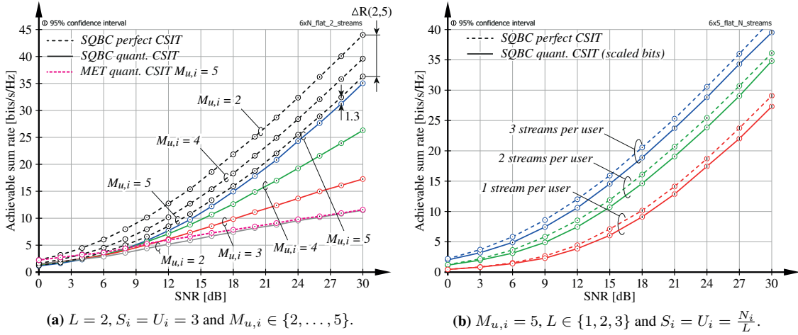
Figure 4.5.: Achievable sum rate of BD-based MU-MIMO systems employing SQBC with quantized and perfect CSIT and N_i = 6 .
