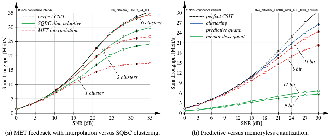
Figure 4.8.: Sum throughput achieved with BD precoding and the proposed limited feedback clustering and quantization algorithms in an N_i \times M_{u,i} = 8 \times 4 system, serving S_i = 4 users over \ell_{u,i} = 2 spatial streams each.
