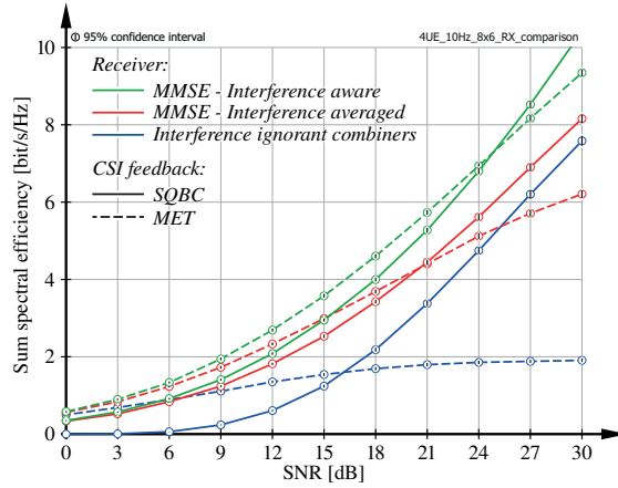
Figure H.1.: Comparison of different combinations of channel subspace feedback strategies and receive equalizers.
