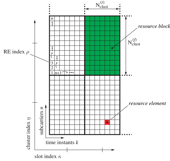
Figure 3.3.: OFDM time-frequency resource grid and clustering of REs into RBs.
