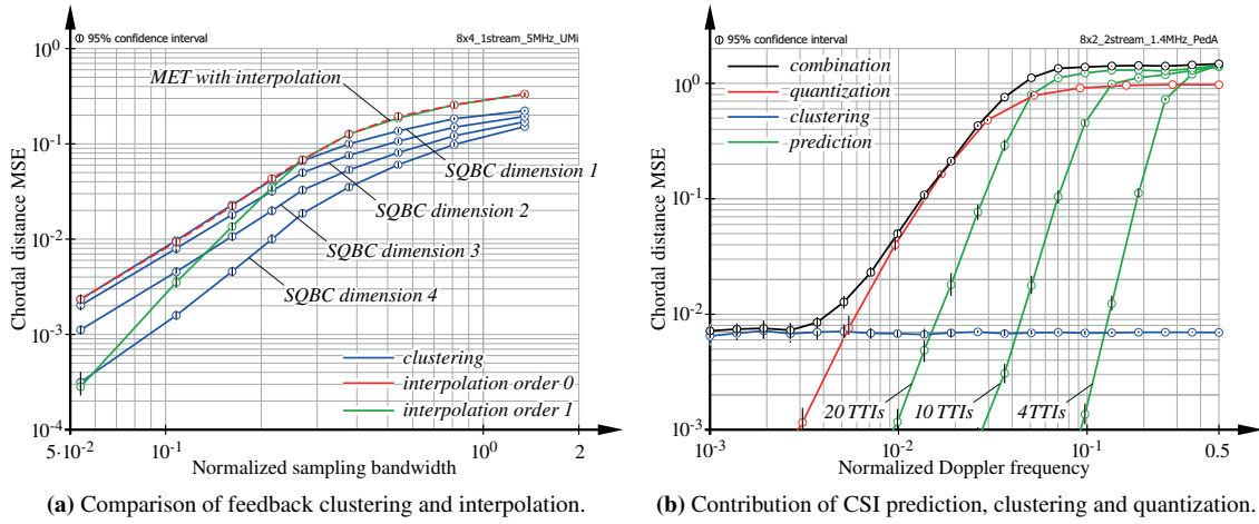
Figure 4.6.: Chordal distance MSE investigation of the proposed CSI feedback methods for frequency-selective channels.
