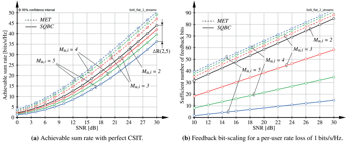
Figure 4.4.: Evaluation of the achievable rate performance and CSI feedback overhead requirement of BD precoding with SQBC and MET antenna combining. Three users are served over six transmit antennas via two streams per user.
