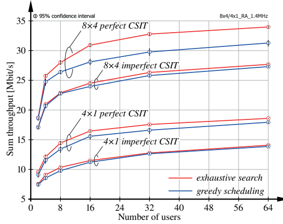
Figure 4.9. Performance of the proposed SUS scheduling algorithm with perfect and imperfect CSIT compared to an exhaustive search. Two configurations are considered: N_i \times M_{u,i} = 4 \times 1 with \ell_{u,i} = 1 and N_i \times M_{u,i} = 8 \times 4 with \ell_{u,i} = 2 .
