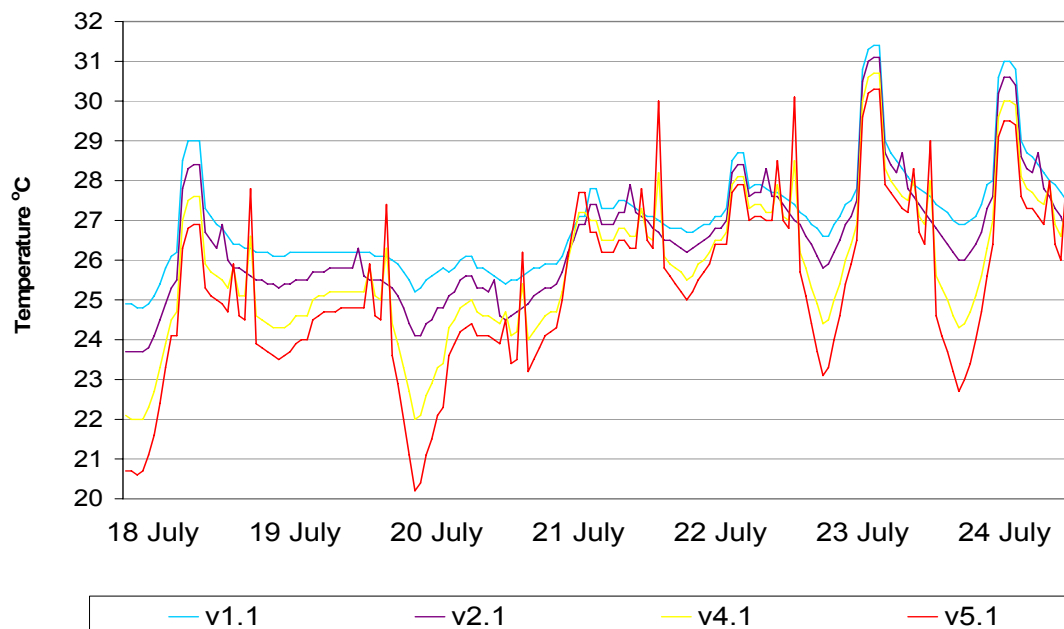
Figure 46: Inside temperature in living room & kitchen (Apartment Vienna) for four ventilation scenarios. Shading scheme: Overhang.
