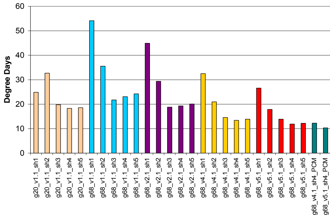
Figure 60: Concentrated results for all parametric studies for the single house in Athens: Test room: Bedroom_2.
