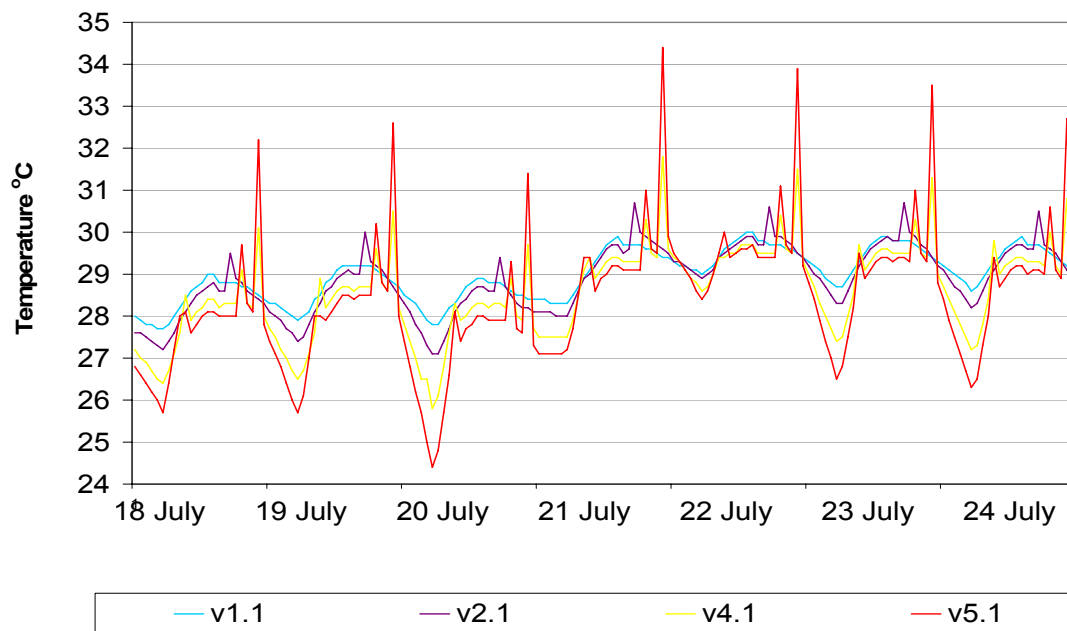
Figure 45: Inside temperature in living room & kitchen (Apartment Athens) for four ventilation scenarios. Shading scheme: External shading device.
