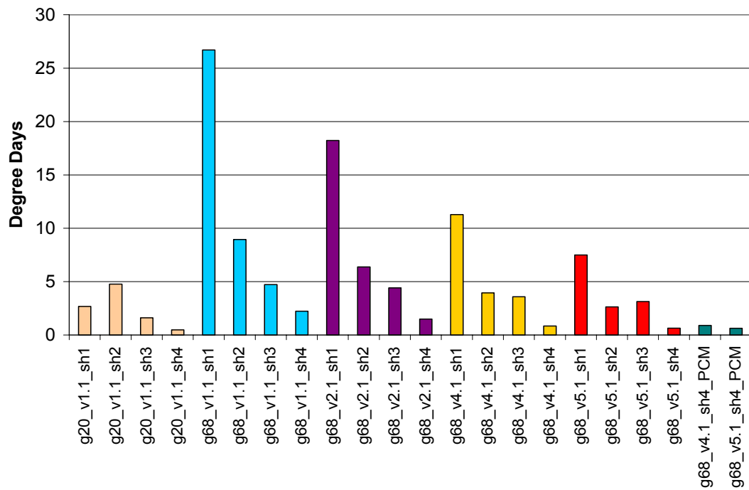
Figure 59: Concentrated results for all parametric studies for the apartment in Vienna: Test room: Living room & kitchen zone.
