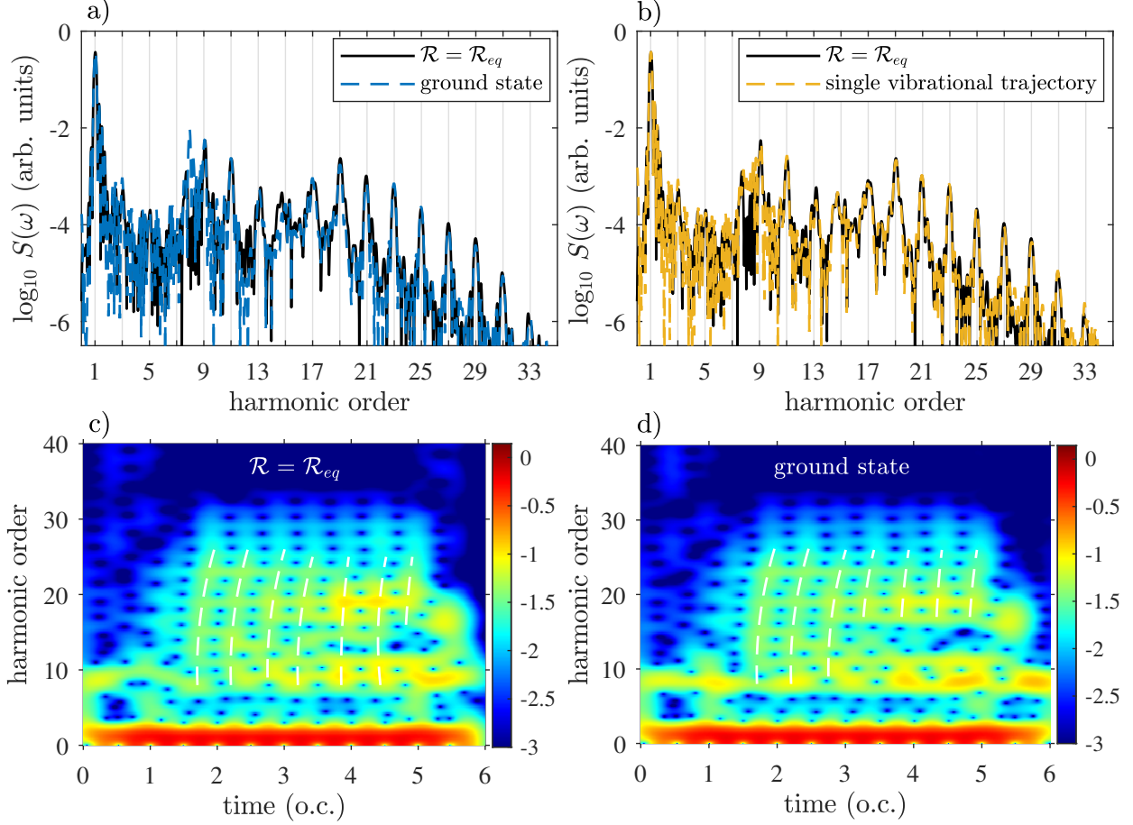
FIG. 6. Harmonic spectrum of F 2 driven by a 6-cycle laser pulse ( \lambda = 800 nm, I_0 = 10^{14} W/cm 2 ). a) Comparison between fixed nuclei at \mathcal{R} = \mathcal{R}_{eq} and sampling over the stationary ground-state wavefunction (Eq. 13). b) Comparison between \mathcal{R} = \mathcal{R}_{eq} and a single Ehrenfest trajectory starting at the outer turning point \mathcal{R}_0(t = 0) = \mathcal{R}_{eq} + |\alpha|\sigma with scaled amplitude |\alpha| = 0.7 . c) Time-frequency analysis of HHG from F 2 for fixed nuclei (black line in panel a) and d) for the sampling over the ground-state wavefunction (blue/gray dashed line in panel a). The temporal width of the Gaussian window function in the Gabor transform is \sigma_\tau = 0.5 fs ( \approx 0.19 o.c.).
