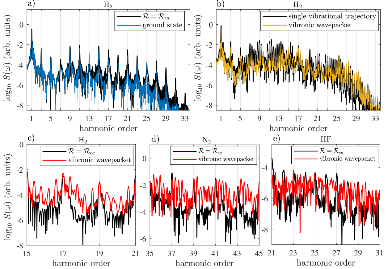
FIG. 7. Harmonics for laser driving frequencies \omega_L commensurate with the frequency \Omega of the vibrational wavepacket. a)–c) \text{H}_2 , d) \text{N}_2 , and e) HF. In frames c)–e) we compare the HHG spectrum for fixed internuclear distance \mathcal{R} = \mathcal{R}_{eq} with the result for the vibrational wavepacket with sampling over the width of the vibrational wavefunction (5 trajectories \mathcal{R}_j(t) ). a) Comparison of complete spectra of \text{H}_2 irradiated with \lambda = 800 nm, I_0 = 10^{14} W/cm 2 , and |\alpha| = 1.8 . black line: fixed-ion calculation for \mathcal{R} = \mathcal{R}_{eq} , blue/dark gray line: vibrational ground-state (Eq. 13). b) As panel a) but calculated using Ehrenfest-TDDFT for single trajectory (black line) and for a vibrational wavepacket sampling by 5 trajectories \mathcal{R}_j(t) (Eq. 19; orange/light gray line), c) zoom-in of a) and b) for high harmonics of \text{H}_2 d) \text{N}_2 with \lambda = 1147 nm, I_0 = 10^{14} W/cm 2 and |\alpha| = 2.8 , e) HF with \lambda = 800 nm, I_0 = 10^{14} W/cm 2 and |\alpha| = 3.25 .
