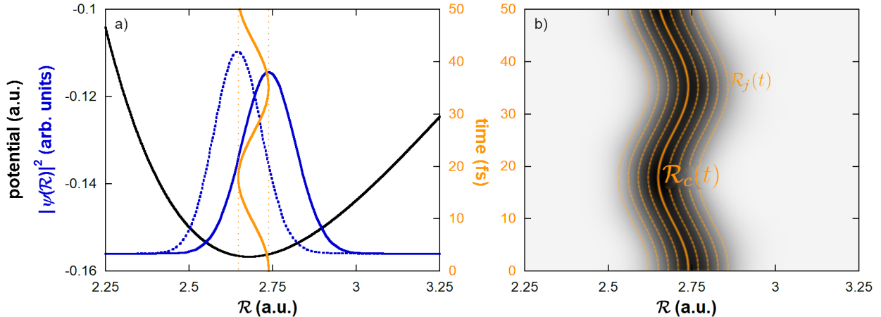
FIG. 1. a) Morse-type molecular potential curve for F_2 (thick black line) and coherent vibrational wavepacket at turning points (dotted and solid blue/dark gray lines). Temporal evolution of expectation value \langle \mathcal{R}(t) \rangle (or Ehrenfest trajectory \mathcal{R}_c(t) , orange/light gray solid line; time in fs on right axis). b) Trajectories \mathcal{R}_j(t) (thin dashed red lines) close to the Ehrenfest trajectory \mathcal{R}_c(t) (thick solid orange/light gray line) sampling the wavefunction of the vibrational wavepacket, schematically.
