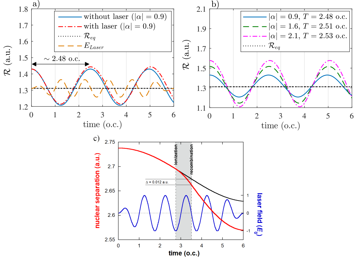
FIG. 2. a) Comparison between the time-dependent internuclear distance \mathcal{R}(t) of \text{H}_2 in the presence (red dash-dotted line) and absence (blue solid line) of the IR laser field ( \lambda = 800 nm, I_0 = 10^{14} W/cm ^2 ) as a function of time in units of optical cycles (o.c.). For illustrative purposes, the amplitude of the laser field is also displayed (in arbitrary units; orange dashed line). For later reference, we note that the frequencies are approximately commensurate, \omega_L/\Omega \approx 5/2 . The equilibrium distance \mathcal{R}_{eq} = 1.31 a.u. predicted by SIC-LDA is also shown for reference. b) Time-dependent \mathcal{R}(t) for field-free evolution predicted by Ehrenfest-TDDFT for varying initial excitation amplitude \mathcal{R}(0) - \mathcal{R}_{eq} = |\alpha| \cdot \sigma to probe for effects of anharmonicity. The legend in the inset denotes the changes of the vibration period. c) Example of a trajectory \mathcal{R}_c(t) for \text{F}_2 in the laser field when \mathcal{R}_c(t) initially follows the mean field but intermittently propagates on the \text{F}_2^+ potential curve (Tully hopping [70]) during the excursion of the electron following tunnel ionization at t = 2.75 optical cycles, acceleration, and recombination at t = 3.5 optical cycles (in red/dark gray). The black line indicates the Ehrenfest trajectory for molecular vibration on the \text{F}_2 potential energy surface without Tully hopping.
