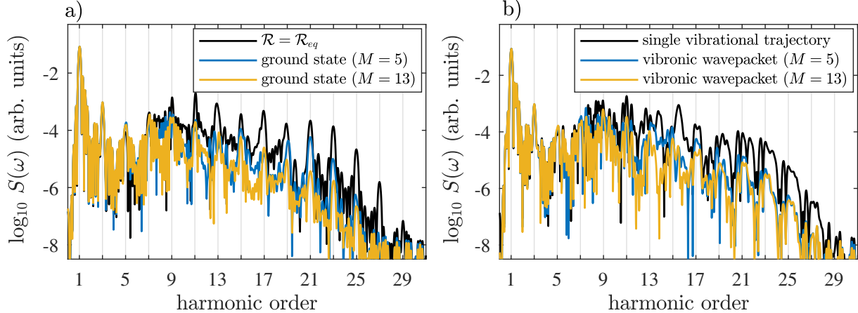
FIG. 3. Harmonic spectra of \text{H}_2 driven by a 6-cycle laser pulse ( \lambda = 742 \text{ nm} , I_0 = 10^{14} \text{ W/cm}^2 ). a) Comparison between spectra for fixed nuclei at \mathcal{R} = \mathcal{R}_{\text{eq}} and for sampling of the vibrational ground-state wavefunction with 5 (blue/dark gray) and 13 (orange/light gray) sampling points \mathcal{R}_i . b) Comparison between single Ehrenfest trajectory \mathcal{R}_c(t) starting at the outer turning point \mathcal{R}_c(t = 0) = \mathcal{R}_{\text{eq}} + |\alpha|\sigma with |\alpha| = 0.9 and sampling over a Schrödinger minimum uncertainty wavepacket with 5 (blue) and 13 (orange) sampling trajectories \mathcal{R}_j(t) .
