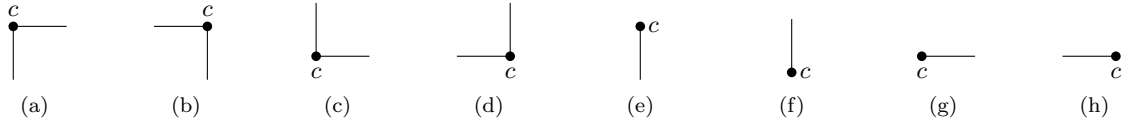
Figure 3: Directions of a reflex corner associated with a degree-2 vertex or with a bend: (a) up-left; (b) up-right; (c) down-left; (d) down-right. Directions of a degree-1 vertex: (e) upward; (f) downward; (g) leftward; (h) rightward.
