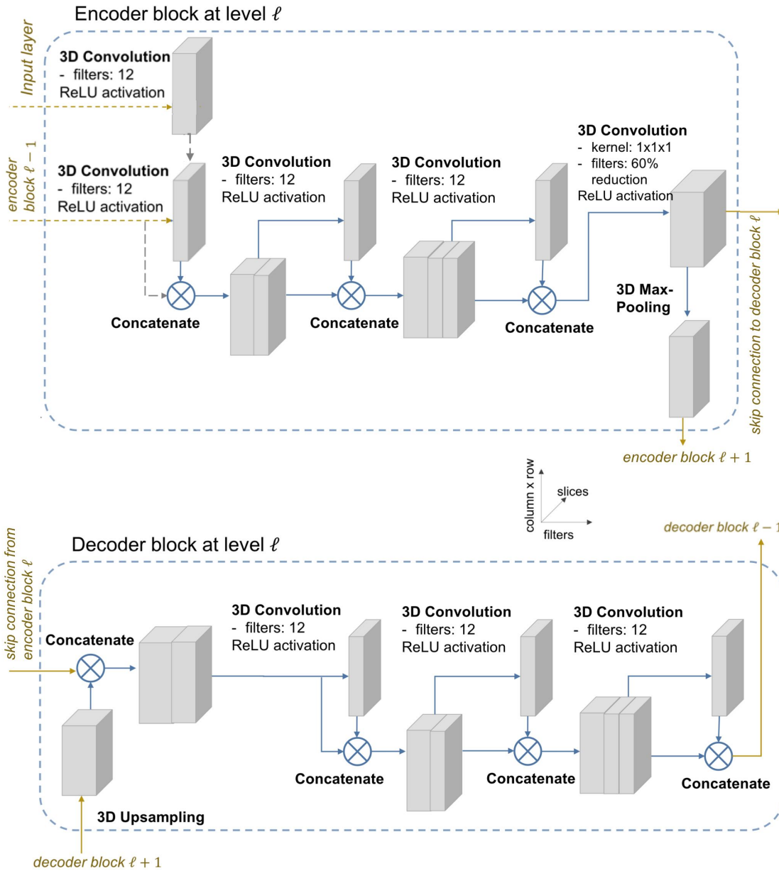
Figure 6.7: FCN_DenseNet: Network architecture of encoder blocks and decoder blocks.
