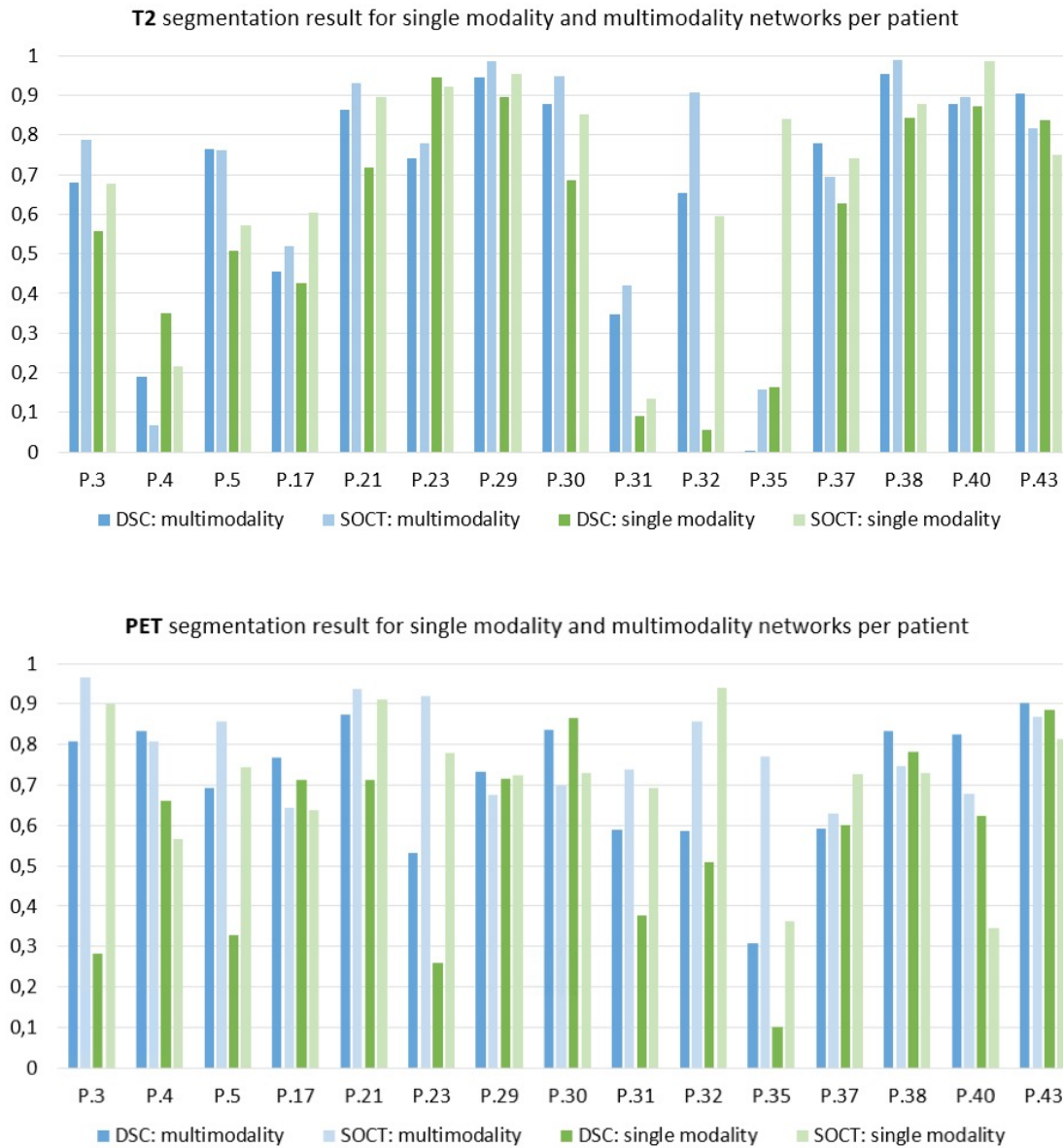
Figure 7.2: Comparison of single modality (T2 or PET) networks and multimodality (T1, T2, and PET) networks, using DSC and SOCT scores per patient. The presented patients are from the first fold of the 3-fold cross-validation.
