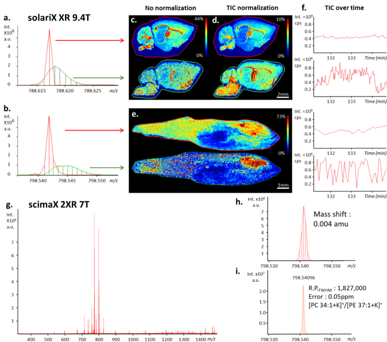
Figure 4. Centroided average MSI mass spectra of mouse brain (a) and zebrafish (b) using a MALDI FT-ICR (solarix XR 9.4T, fitted with ParaCell) instrument, zoomed in on m/z 788.62 and 798.54, respectively, showing peak width differences due to MMA obtained with (red) and without (green) TIC stabilization by optimization of the laser shot number (6 laser shots at 60 Hz). Reconstructed brain slices MS images without (c) and with (d) TIC normalization. Reconstructed zebrafish whole-body slices MS images with TIC normalization (e, TIC stabilization method (up) and no TIC stabilization (down), respectively). Section of the TIC over time to show the TIC stability of the presented MSI (f). Centroided average MSI mass spectrum of a mouse brain tissue section acquired on the scimaX 2XR using the 2\omega detection mode with TIC stabilization (g). Zoom in to m/z 798.54 showing peak width difference due to MMA (h). Zoom in on m/z 798.54 in an extracted pixel spectrum showing the obtained R.P., FWHM and MMA (i). See text for details.
