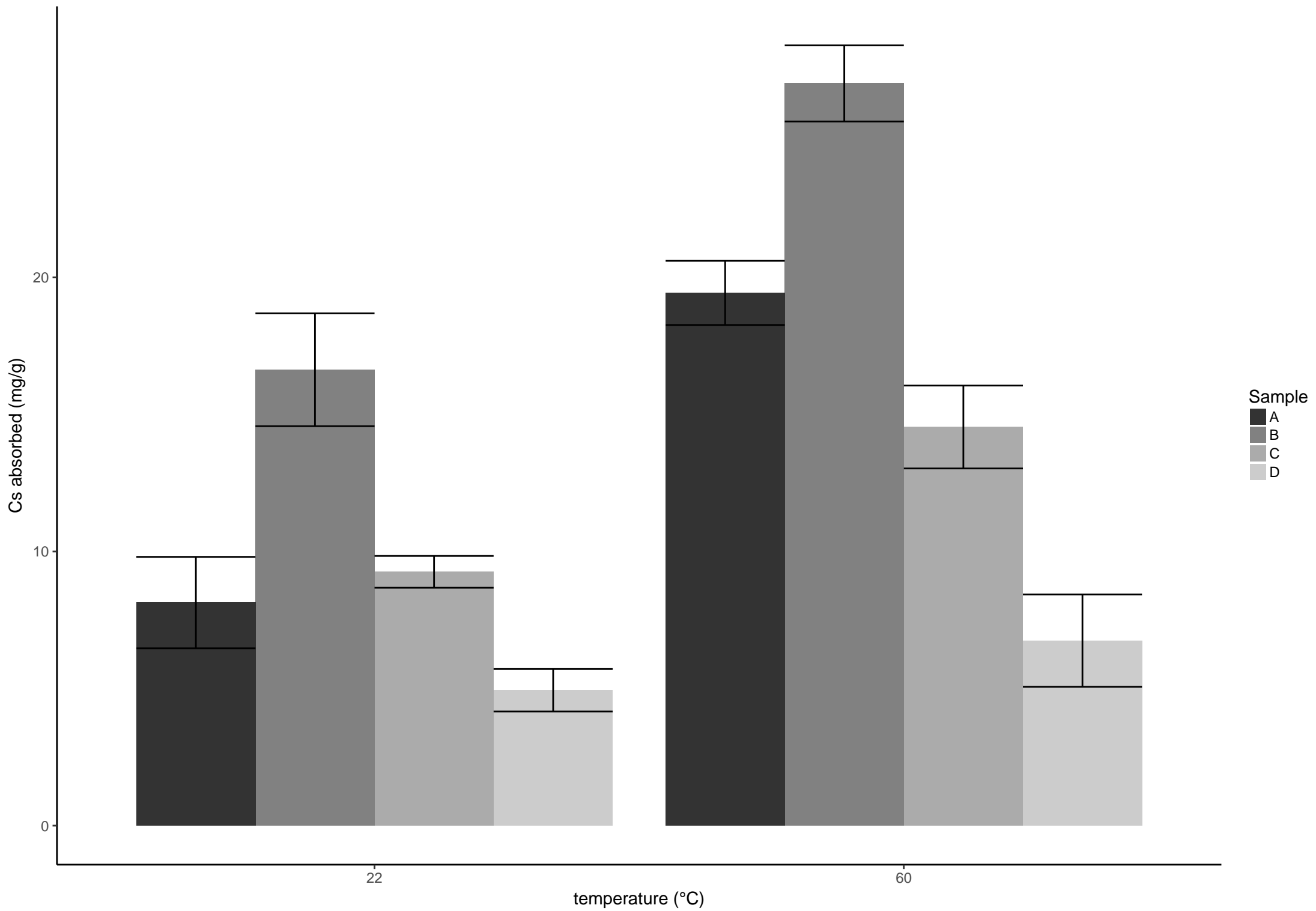
Absorbed Sr by Temperature (5 mins)
