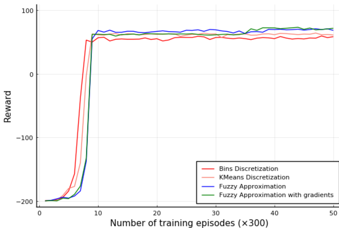
Figure 4.2: Evolution of rewards obtained through training for 4 algorithms (results are averaged over 300 runs)
