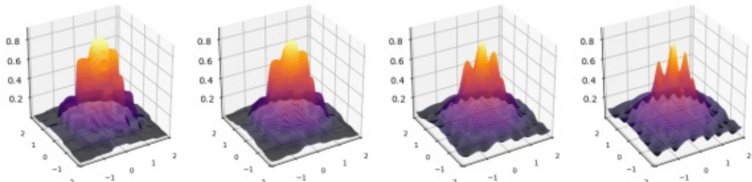
Figure 3.4: Fuzzy approximation for different values of the fuzzifier (from left to right: 1.2, 1.5, 1.8, 2)
