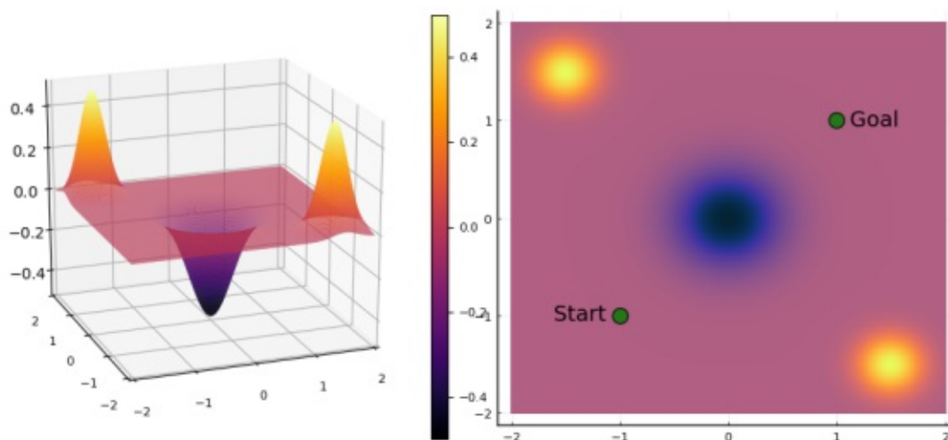
Figure 4.1: The test environment (left: the surface on which the object evolves; right: heatmap representation)
