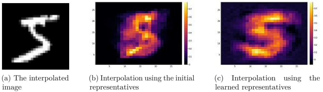
Figure 5.5: Fuzzy interpolation of a digit. Interpolated images are represented through heatmaps for scale and readability.
