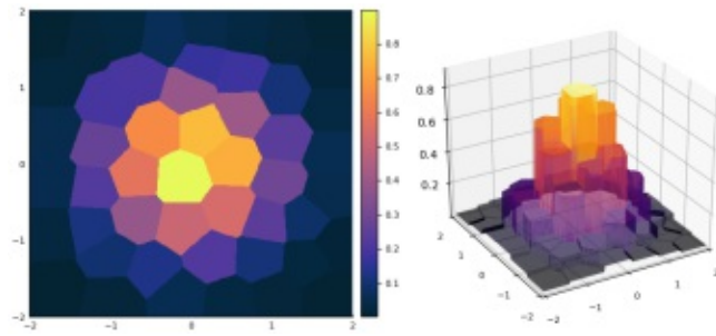
Figure 3.2: Piece-wise constant approximation ( E \approx 0.072 )
