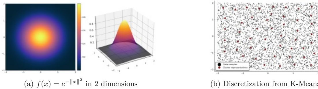
Figure 3.1: A test case for cluster-based function approximation
