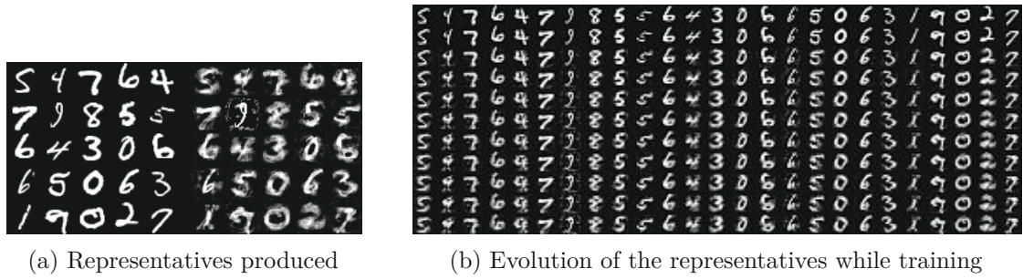
Figure 5.4: Representatives produced after 1 epoch of training, when initializing with k-means++. (a) Initial representatives (left) compared with learned representatives (right); (b) some representatives change shapes while training.
