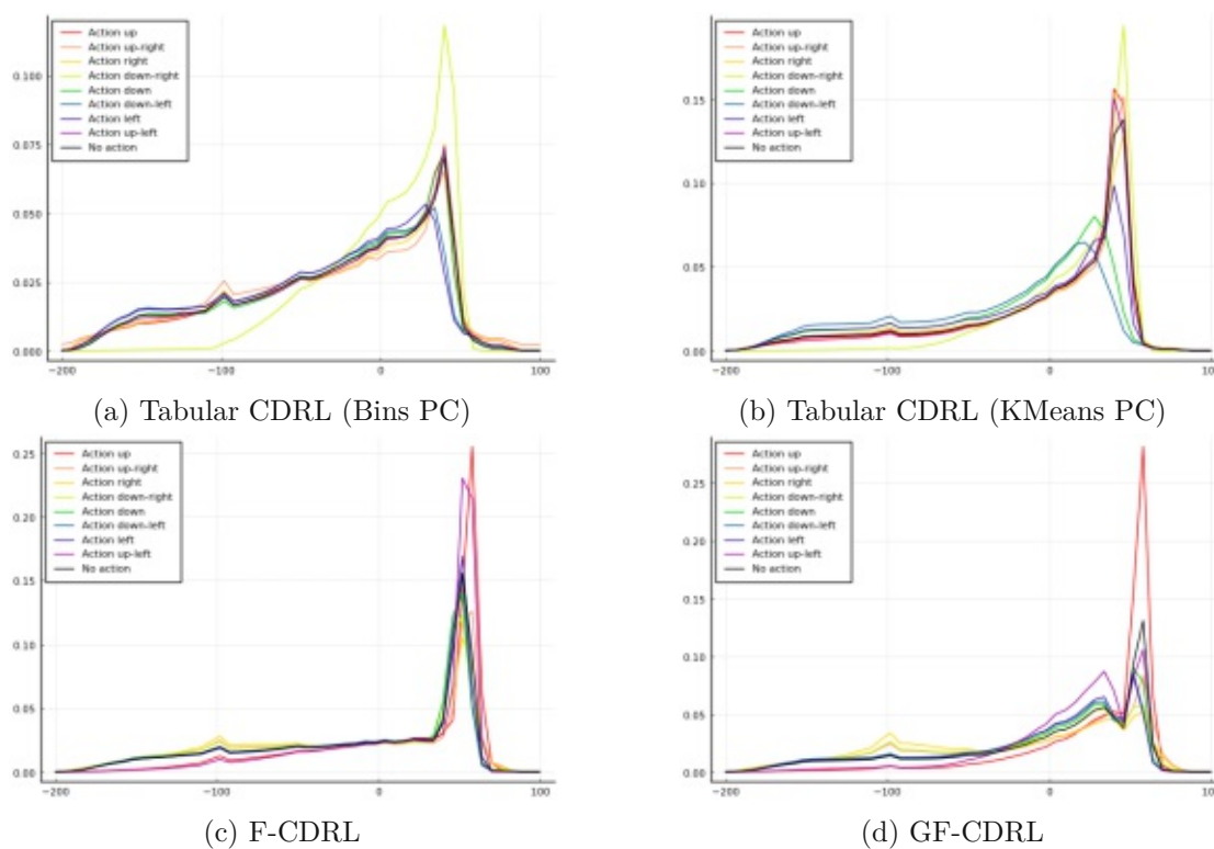
Figure 4.4: Learned action-value distribution at the initial state for the different algorithms.
