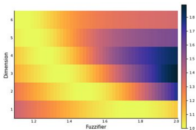
Figure 3.6: Approximation error as a function of dimension and of the fuzzifier
