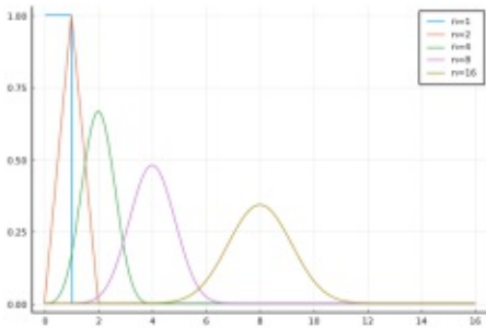
(a) Irwin-Hall distribution
