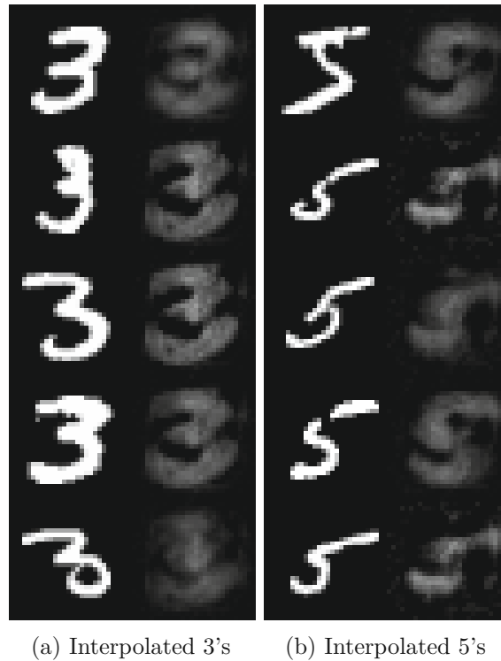
Figure 5.3: Results of the fuzzy interpolation of some images by the learned memberships layer. For each pair of digit, the left one is the actual data sample and the right one is the interpolated one.
