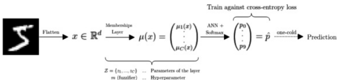
Figure 5.1: The considered network architecture
