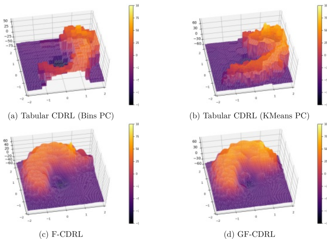
Figure 4.3: Maximal expected value of action-value distribution for the different algorithms.
