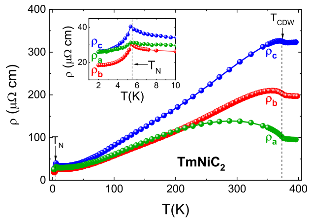
FIG. 3. Temperature dependent electrical resistivity measured with applied current along orthorhombic a (green), b (red) and c (blue) orientations of \text{TmNiC}_2 single crystal bars; solid lines are guides to the eye. Inset zooms towards the AF transition. Both CDW and AF transitions are indicated by the black arrows and dotted lines.
