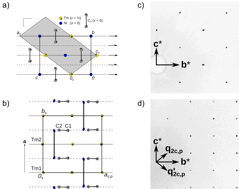
FIG. 1. a) The high-temperature phase of \text{TmNiC}_2 at 400 K viewed down [100] . Tm (yellow), Ni (blue) and C (gray) atoms are represented by ellipsoids drawn at the 75% probability levels. Symmetry operations of the Amm2 space group are indicated using the usual graphical symbols [33]. A gray backdrop indicates the unit cell of the low-temperature superstructure. b) The low-temperature phase of \text{TmNiC}_2 at 280 K viewed down [001] (corresponding to the [01\bar{1}] direction of the high-temperature phase). The indicated unit-cell corresponds to the conventional setting of the low-temperature phase. A p -subscript indicates a vector pointing out of the drawing plane. The lattice basis vector \mathbf{a} of the aristotype is indicated. c) h = 0 and d) h = \frac{1}{2} sections of reciprocal space of a \text{TmNiC}_2 crystal at 280 K reconstructed from single crystal XRD frame data. The reciprocal basis of the basic structure and the modulation vectors of both twin domains are indicated. A subscript ‘p’ designates a vector projected onto the drawing plane.
