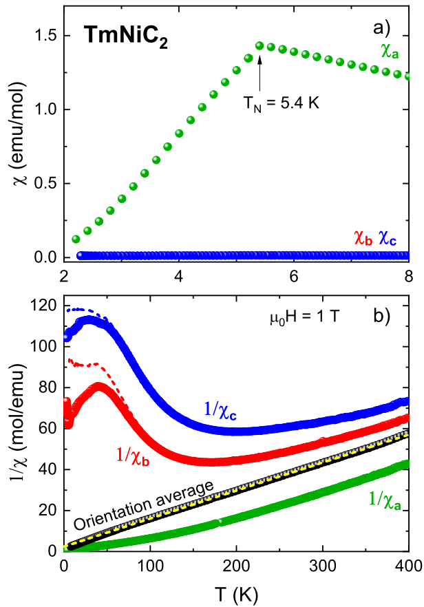
FIG. 5. a) The temperature dependent dc magnetic susceptibility of single-crystalline TmNiC 2 measured along the orthorhombic a -axis orientation with an applied magnetic field of 63 mT and along the b - and c -orientations with a field of 0.1 T; b) corresponding inverse dc susceptibility, 1/\chi , shown for principal orientations, all measured at 1 T. The original data are shown as symbols and data of 1/\chi_b and 1/\chi_c corrected with respect to an obvious misalignment of the measured crystal (see text) are presented as dashed lines.
