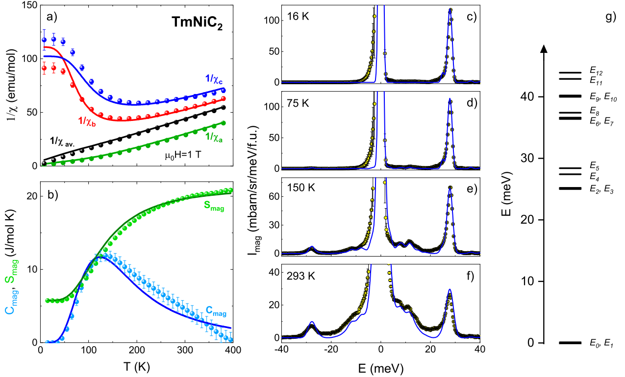
FIG. 7. a) CEF fitting of alignment corrected inverse magnetic susceptibility data of single-crystalline \text{TmNiC}_2 ; b) of magnetic heat capacity and magnetic entropy contributions (solid lines are fits); and c-f) of magnetic scattering functions I_{\text{mag}}(\omega) measured at four different temperatures, where error bars of data points representing the quasi-elastic line are artificially enlarged by orders of magnitude in order to effectively exclude the quasi-elastic line from the fitting process; blue solid lines are calculated I_{\text{mag}}(\omega) functions obtained by Gaussian convolutions of the calculated magnetic scattering intensities (see text for details of the temperature variation of the applied half widths); g) resulting CEF energy level splitting.
