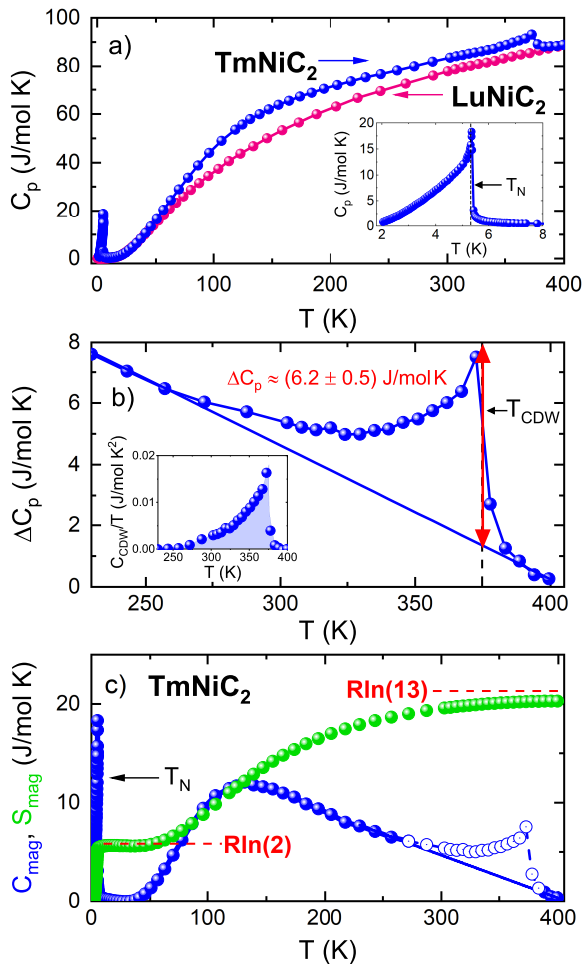
FIG. 4. a) Temperature dependent specific heat of \text{TmNiC}_2 (blue) and \text{LuNiC}_2 (pink) where lines connecting data points are just guides to the eye; the inset zooms in on the AF transition; b) \Delta C_p in the vicinity of the CDW transition where the straight solid line serves to extrapolate the CEF Schottky anomaly; the inset shows our estimate of the contribution C_{\text{CDW}}/T (see text); c) temperature dependent magnetic specific heat and entropy contributions where red dotted lines mark S = R \ln(2J + 1) for J = 1/2 and J = 6 , respectively.
