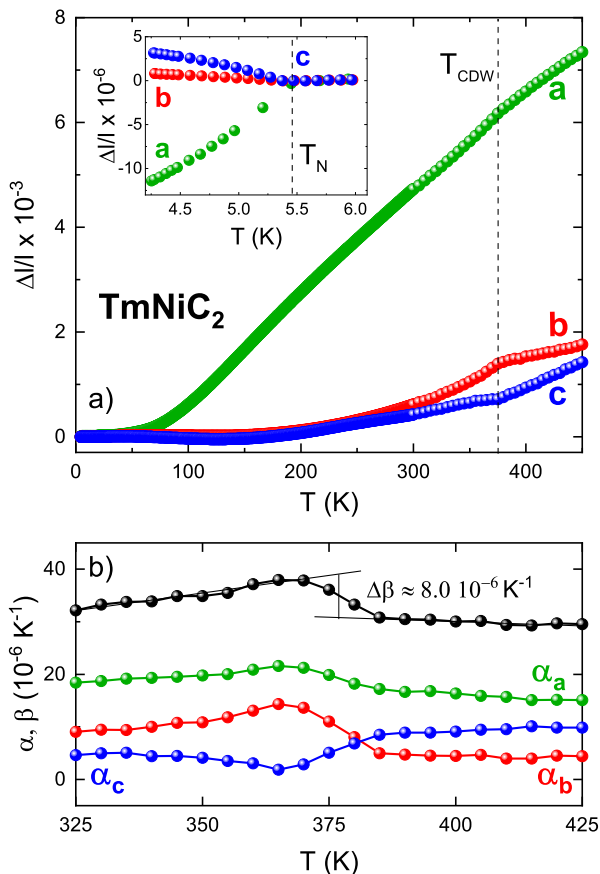
FIG. 2. a) Temperature dependent thermal expansion along orthorhombic a (green), b (red) and c (blue) orientations of \text{TmNiC}_2 . Inset zooms towards the AF transition. Both, CDW and AF transition temperatures are indicated by dotted lines; b) thermal expansion coefficients and volume expansion coefficient vs. temperature. Solid lines are a guide to the eye.
