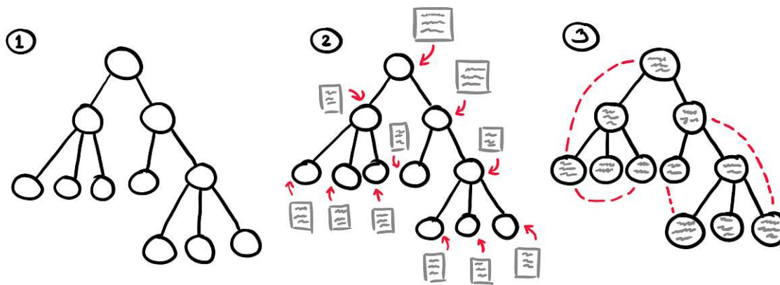
Figure 6.4: The three steps in story graph foraging. First, we build the structural skeleton. Second, we associate textual descriptions with individual nodes. Finally, we add functional relationships.
