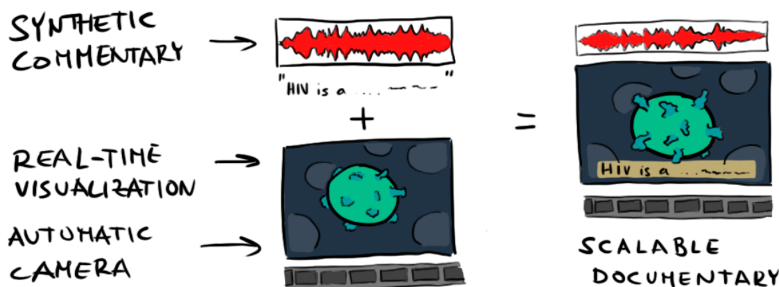
Figure 6.2: The Scalable Documentary concept: We provide visuals as a real-time visualization and couple it with an automatic camera traversing the 3D scene. We augment the fly-through with a synthetic commentary that we generate on-demand, as opposed to using a pre-recorded voice-over.
