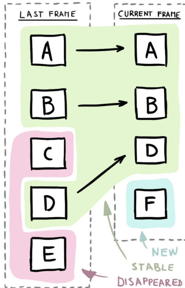
Figure 4.6: Matching of labels across two frames.
