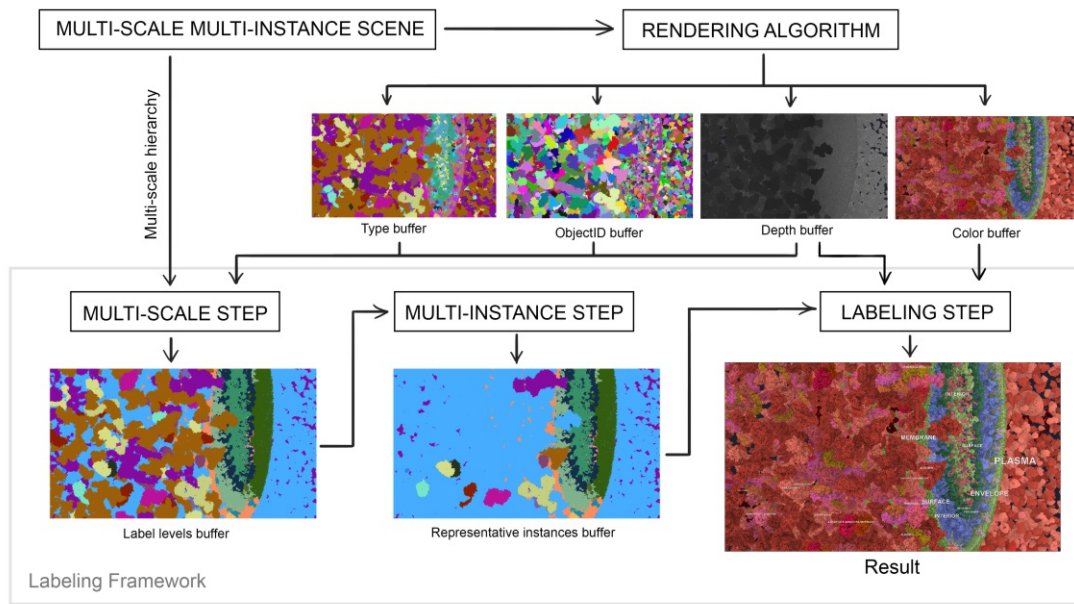
Figure 4.3: Overview of the Labels on Levels (LoL) framework. The multi-scale step utilizes the G-buffer result of a rendering algorithm with the scene’s hierarchy in order to generate depth-aware regions that are to be labeled. Afterwards the multi-instance step selects a representative instance together with a label anchor point inside the chosen instance, which is optimal according to specified criteria.
