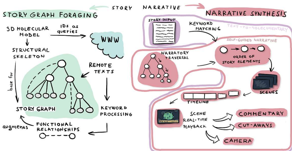
Figure 6.3: Overview of the framework for generating molecumentaries. In describing the technical contributions we follow the distinction between a story (static representation of story elements) and a narrative (dynamic arrangement of these story elements). Story-graph foraging provides a scalable approach for compiling information about the model which can be used for storytelling, while the real-time narrative synthesis encompasses solutions for turning the story graph into a specific narrative at runtime.
