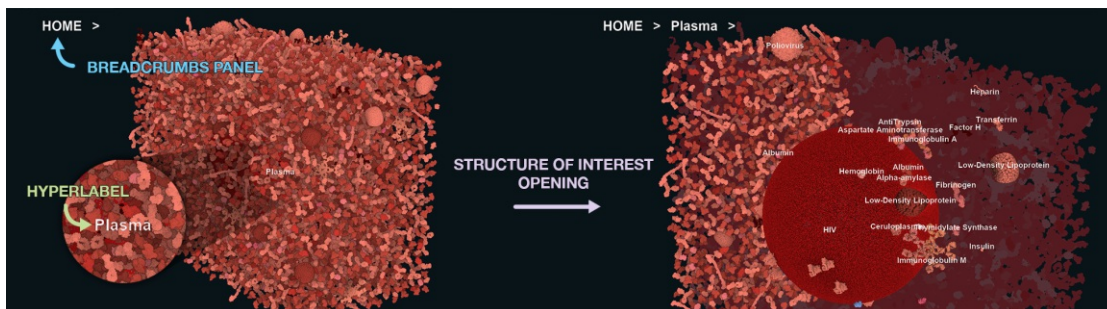
Figure 5.2: Overview of the three components of our method: HyperLabels trigger the operation of Structure of Interest Opening, which adjusts the visibility of the model to allow further exploration. This way the model is traversed in a top-down fashion. The breadcrumbs panel provides orientation and enables navigation in the opposite, bottom-up, direction.
