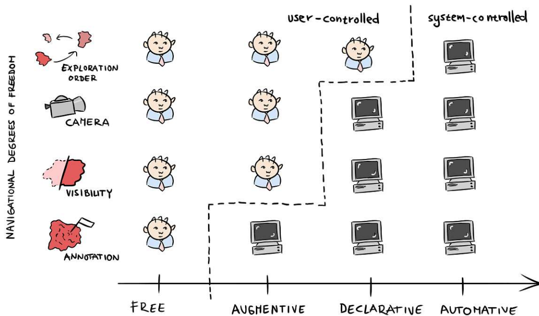
Figure 3.5: Overview of the navigational modes framework. Each of the modes—augmentive, declarative, and automative—are defined as a combination of navigational degrees of freedom given either directly into the user’s hands or entrusted to an automated approach on the visualization system’s side.
