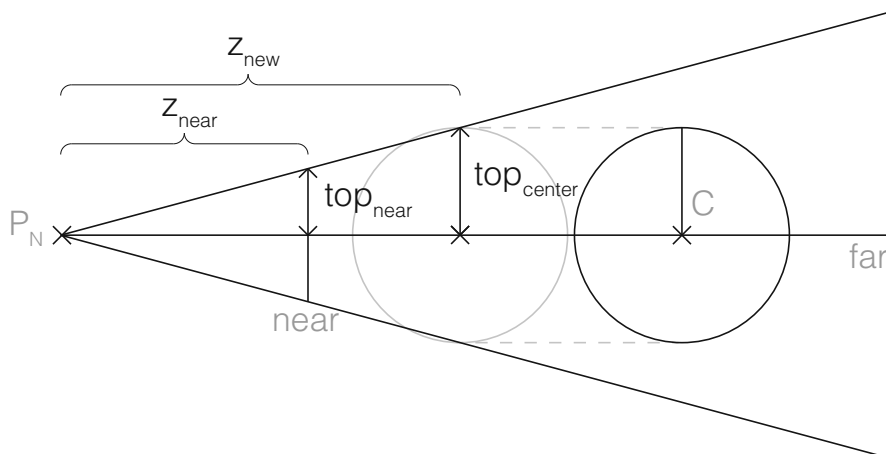
Figure 5.7: To show all objects of the current hierarchy level, we enclose them with a bounding sphere. We then move the camera such that the view frustum touches the top (and bottom) points of the bounding sphere.
