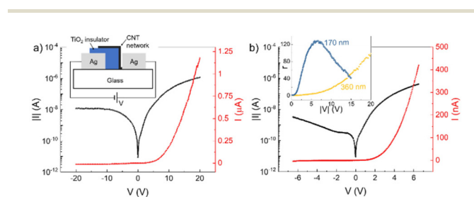
Fig. 4 (a) I - V characteristics of a printed MIS diode on both a semi-logarithmic (left axis, black curve) and linear (right axis, red curve) scale. The average TiO 2 -NS thickness is 360 nm. The inset shows a sketch of the longitudinal section of the structure. (b) I - V characteristics of a nominally identical printed MIS diode but with an average TiO 2 -NS thickness of 170 nm. The inset shows the rectification ratio as a function of the modulus of the applied voltage for the two diodes with different TiO 2 -NS thicknesses. The active area of the diodes is approximately 200 \mu\text{m} \times 100 \mu\text{m} .
