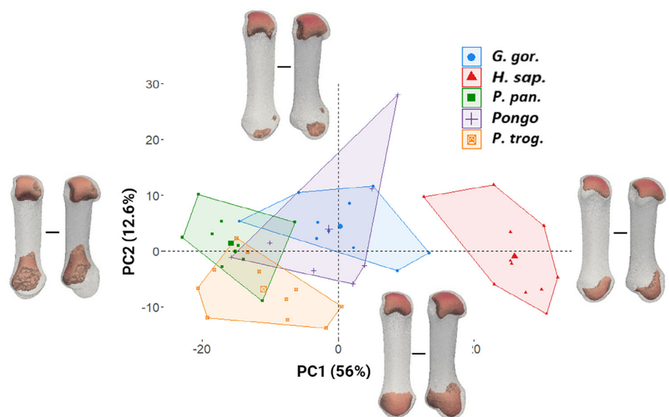
FIGURE 4 PCA of the rBV/TV patterns throughout the whole Mc1. Larger points denote the centroid of each species. The canonical trabecular volumes are colored by the signed loadings at two standard deviations (SD) of each principal component and thresholded at the 75th percentile of this range, to demonstrate volumetric trabecular structure. The volumes are within a translucent canonical mesh of cortical bone and given in palmar (left) and ulno-palmar (right) views.
