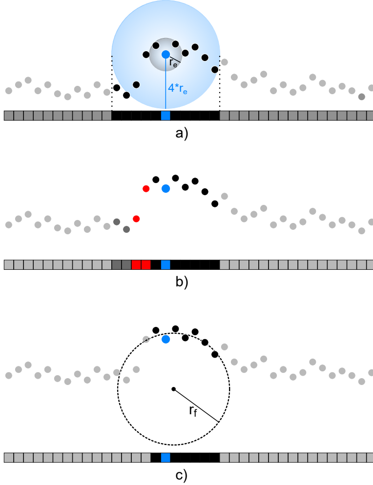
Figure 3.6: Sphere fitting procedure (assuming orthogonal projection for simplicity) for one point p (blue). The 3D neighborhood determined by the point error of p by splatting a sphere of radius 4*r_e to image space (a). Floodfill with p as seed pixel is performed to filter out occlusion points (b). A sphere is fitted to the remaining neighborhood (c).
