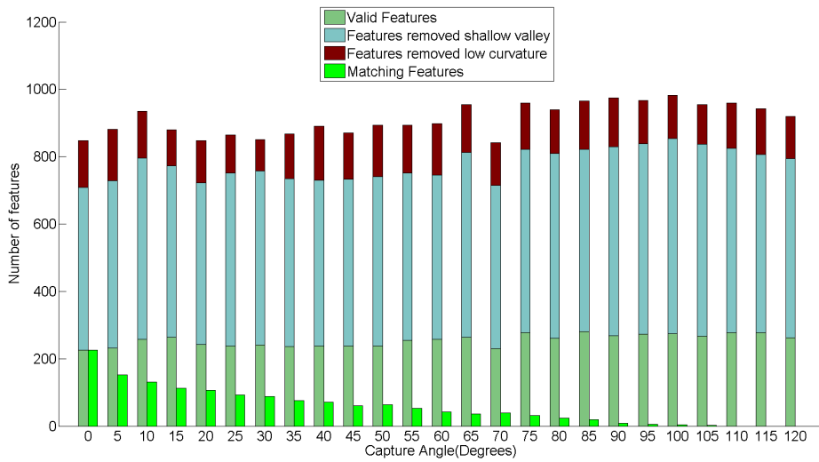
Figure 4.8: Feature counts for the atom model. The total amount of salient points detected averages to 911.04 over all viewing-angles. From the total amount of salient points, on average 133.8 were removed because of a curvature response below 13. From the remaining points another 522.36 were discarded due to having a point in their close vicinity that had a higher curvature response. As can be seen from the depicted ground-truth feature matches, 74 feature matches get lost when rotating the capture angle by the first 5 degrees, but after that, the amount of feature matches deteriorates slowly, and only at an angle difference of 110 degrees, no features could be matched anymore. On average 6.61 feature matches are lost at each capture step.
