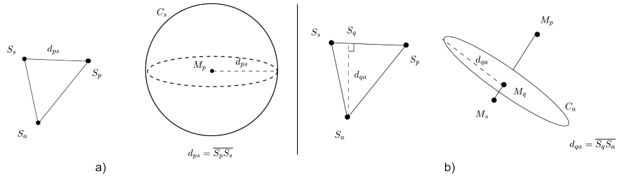
Figure 2.5: The rigidity constrained search in RANSAC-based DARCES for three control points S_p , S_s and S_a . a) shows the initial setup of the primary point S_p , the secondary point S_p and the auxiliary point S_a on the left. How the corresponding point M_s for the secondary point is found once a correspondence candidate M_p for the primary point is chosen, is depicted on the right side. A sphere of radius d_{ps} is centered at M_p and all points at the intersection border of the sphere and the surface are possible candidates for the secondary point. b) shows how to get the corresponding point of the auxiliary point. Image courtesy of Chen et al. [7].
