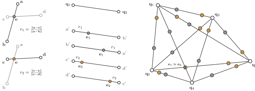
Figure 2.7: Identifying congruent 4-points in a target surface Q . Given a base of 4 roughly coplanar points a, b, c, d calculate ratios r_1 and r_2 (left). With a point pair (q_1, q_2) \in Q , calculate intersection point candidates for each ratio for both directions (middle). 2 point pairs for which intersection points for the correct ratio coincide can be considered for congruency test (right).
