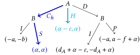
Figure 1: Simplified Closing Game with \alpha, a, \epsilon, f, d_A > 0 and \alpha, \epsilon infinitesimals.
