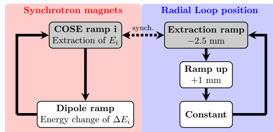
Figure 2: MEE with bunched COSE at MedAustron. The extraction phase is depicted with grey nodes, the energy change phase with white nodes.
