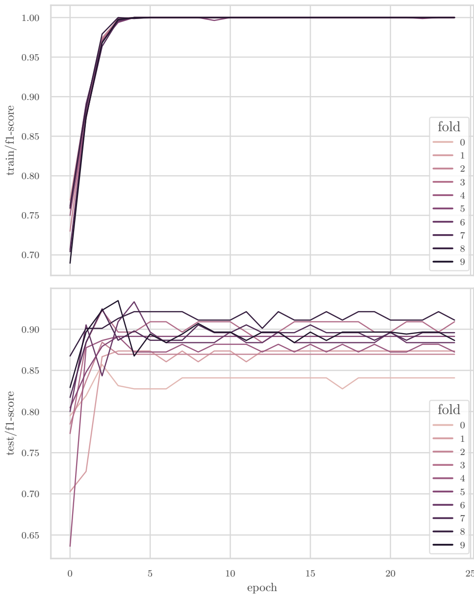
Figure 5.4: These plots show the F_1 -score during training as well as testing for each of the folds. The classifier converges to 1 by the third epoch during the training phase, which might indicate overfitting. However, the performance during testing increases until epoch three in most cases and then stabilizes at approximately 2-3 percentage points lower than the best epoch. We believe that the third, or in some cases fourth, epoch is detrimental to performance and results in overfitting, because the model achieves an F_1 -score of 1 for the training set, but that gain does not transfer to the test set. Early stopping during training alleviates this problem.
