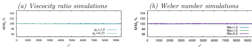
FIGURE B.1 – Mass conservation for the different two-layer flow simulations. Left: simulations at variable viscosity ratio, right: simulations at variable Weber number.
