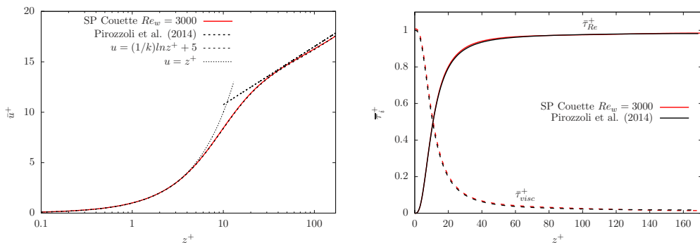
FIGURE A.1 – Mean velocity profile (left) and stress behaviour (right) from the simulation of the single-phase Couette flow. Results are compared to those of Pirozzoli et al. [172].
