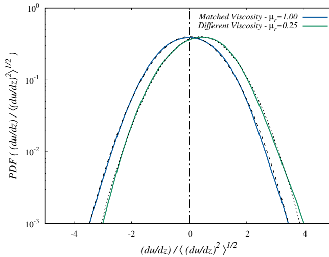
FIGURE 2.3 – Probability density function of the normalized strain rate du/dz / \langle (du/dz)^2 \rangle^{1/2} for cases \mu_r = 1.00 (blue line) and \mu_r = 0.25 (green line). The Gaussian distributions with mean values \alpha = 0 , \alpha = 0.4 and unit standard deviation are shown with a dashed and a dotted black line respectively.
