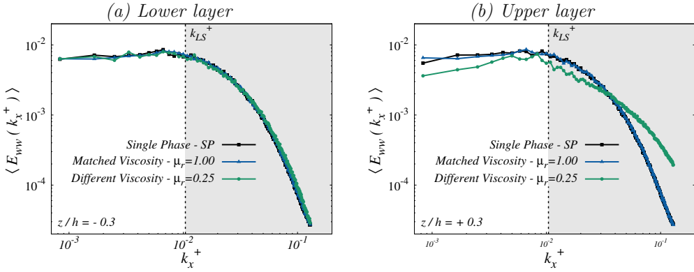
FIGURE 2.7 – Streamwise wavenumber spectrum of the vertical velocity fluctuations, E_{ww} , averaged in time, computed on wall-parallel planes x-y below the interface (at z/h = -0.3 , panel a) and above the interface (at z/h = 0.3 , panel b). Results for \mu_r = 1.00 and \mu_r = 0.25 are shown together with the results obtained for the reference single-phase flow.
