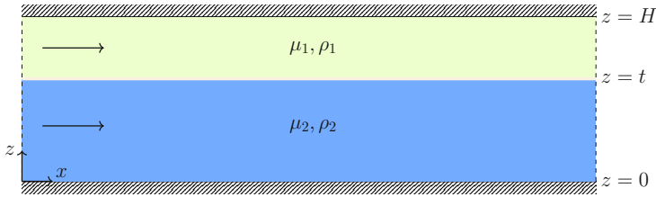
FIGURE 1.8 – Two fluid layers flowing in parallel in a rectangular channel driven by the action of a mean pressure gradient. The arrows indicate the flow direction.
