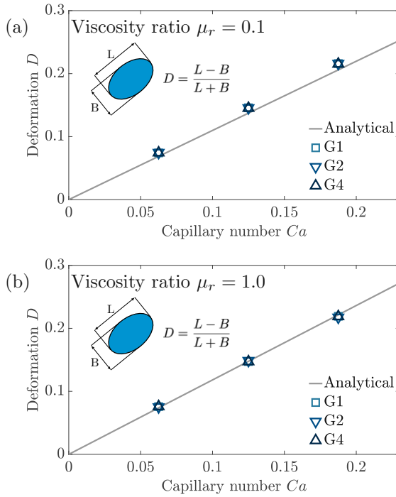
FIGURE 1.11 – Behaviour of the deformation parameter D (see sketch) as a function of the Capillary number, Ca , for a drop in a two-dimensional shear flow: comparison between the numerical results (symbols) and analytical predictions (continuous black lines). Two different viscosity ratios are considered: \mu_r = 0.1 (panel a) and \mu_r = 1.0 (panel b). The different symbols refer to the different refinement factors employed: light blue squares (case G1), blue down-facing triangles (case G2), upward-facing dark blue triangles (case G4).
