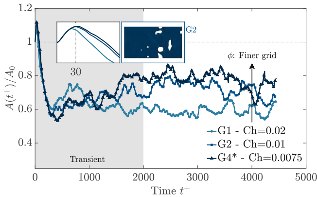
FIGURE D.3 – Evolution of total interfacial area A(t^+) , normalized by the initial area A_0 . Results from the three simulations G1 , G2 and G4^* are shown using different colors, from light to dark blue. The grey area represents the initial transient, after which a statistically steady condition is reached.
