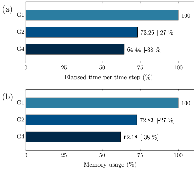
FIGURE 1.12 – Computational efficiency of the dual-grid approach: elapsed time (wall-clock) for a time step (panel a) and memory usage (panel b). Results are normalized using case G1 as reference, where the finest grid is used for all equations. Light blue bars refer to case G1 (same grid), blue bars to case G2 (refinement factor equal to 2) and dark blue bars to case G4 (refinement factor equal to 4).
