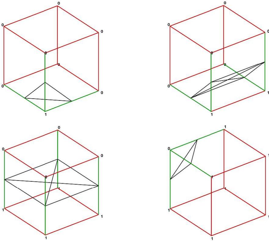
FIGURE 1.7 – Different polygon configurations emerging in the marching cubes algorithm triangulation step. The bit values 0 and 1 can be seen on the vertices of the cube. The polygon edges, shown in black, connect the midpoints of edges with different digits at their vertices. The connected edges are colored in green contrary to the unconnected edges, which are colored in red.
