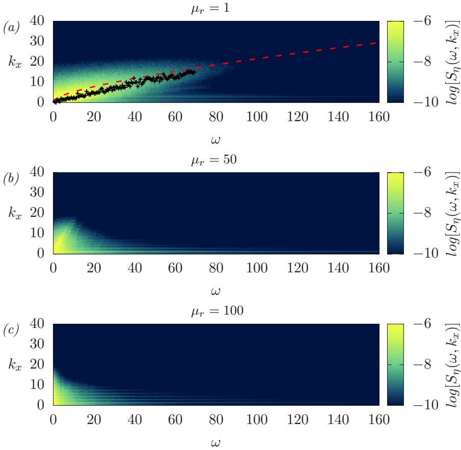
FIGURE 3.11 – Frequency-wavenumber power spectra of wave elevation for \mu_r = 1 (panel a), \mu_r = 50 (panel b), \mu_r = 100 (panel c). The dashed red line corresponds to the Linear Dispersion Relation (LDR) for capillary waves while the black crosses correspond to the maxima of the numerical results.
