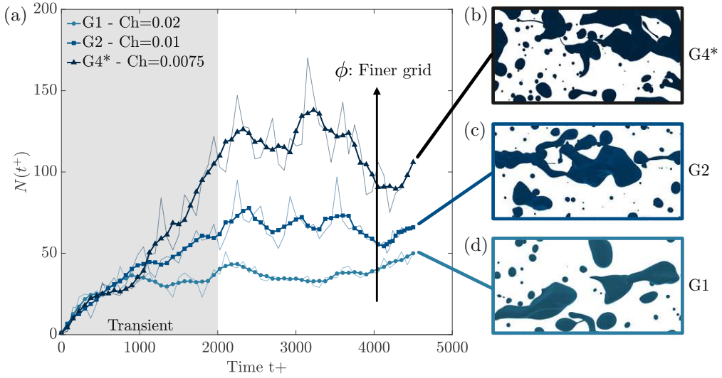
FIGURE D.4 – Time behaviour of the number of drops, N(t^+) , for the three simulations considered here, ( G1 , G2 and G4^* ). The shaded area indicates the extension of the initial transient, after which a steady-state condition is reached ( t^+ > 2000 ). Qualitative pictures (panels b-d), show a snapshot of the drops near the channel center, at the end of the simulation ( t^+ = 4500 ).
