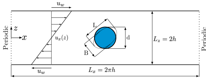
FIGURE 1.10 – Sketch of the deformation of a drop in a shear flow. A circular drop of diameter d = 0.8h is initially located at the centre of the channel (blue circle). The domain is two-dimensional with dimensions L_x \times L_z = 2\pi h \times 2h . Periodicity is applied along x , and the two walls move in opposite directions with constant velocity u_x = u_w = \pm 1 . The imposed shear deforms the drop into an ellipsoid (a qualitative representation of its final shape is given by the dotted line). Drop deformation is evaluated computing the deformation parameter D = (L - B)/(L + B) , being L and B the major and minor axes of the ellipsoid, respectively.
