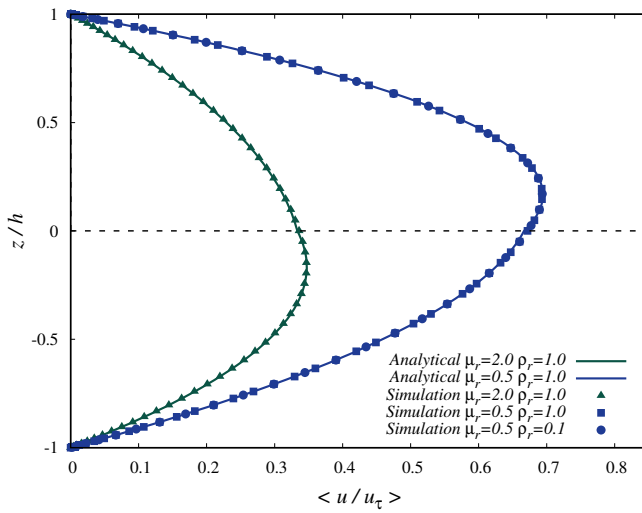
FIGURE 1.9 – Comparison between analytically calculated and numerically computed mean velocity profiles of a two-layer Poiseuille flow for two different values of the viscosity ratio, \mu_r = 2.0 and \mu_r = 0.5 , and two different values of the density ratio, \rho_r = 1.0 and \rho_r = 0.1 .
