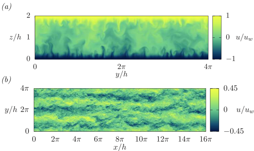
FIGURE A.2 – (a) Instantaneous map of the streamwise velocity, u over the cross-section of the channel. (b) Instantaneous map of the streamwise velocity, u over the horizontal centerplane z/h = 1 .
