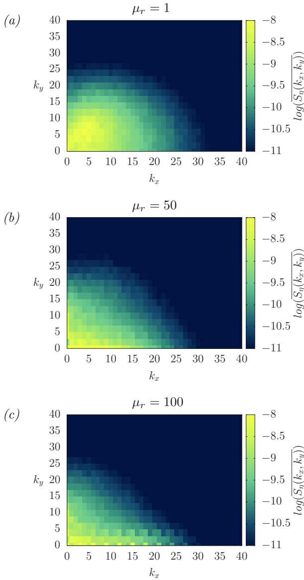
FIGURE 3.8 – Two-dimensional time-averaged wavenumber power spectra of the interface elevation, \overline{S_\eta(k_x, k_y)} . Each panel refers to a different case: \mu_r = 1 (panel a), \mu_r = 50 (panel b), \mu_r = 100 (panel c).
