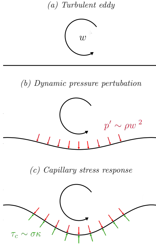
FIGURE 2.8 – Wave generation by turbulence. Panel (a) : a turbulent eddy encounters the undeformed interface at t = 0 . Panel (b): the interface deforms as a result of the dynamic pressure, p' . Panel (c): capillary stress, \tau_c resists the deformation.
