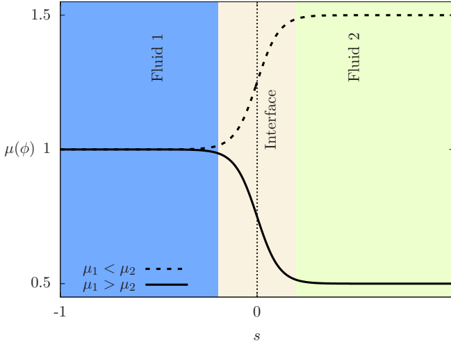
FIGURE 1.2 – Viscosity profile across the two fluid phases separated by a flat interface as a function of the interface normal coordinate s , for two different values of the viscosity ratio.
