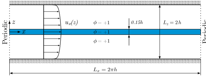
FIGURE D.1 – Sketch of the simulation setup used to simulate the breakage of a liquid layer in a turbulent channel flow. A thin liquid layer, thickness 0.15h , is initially placed at the center of a three-dimensional turbulent channel (the initial shape and location of the layer are represented in blue). The domain is three-dimensional, with dimensions L_x \times L_y \times L_z = 2\pi h \times \pi h \times 2h .
