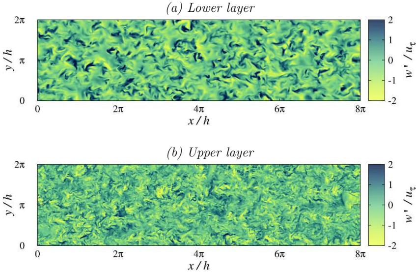
FIGURE 2.6 – Contour-maps of wall-normal velocity fluctuations, w , on wall-parallel x-y planes located near the interface, for the case \mu_r = 0.25 . Panel (a): x-y plane below the interface, in the lower layer, at z/h = -0.3 . Panel (b): x-y plane above the interface, in the upper layer, at z/h = 0.3 .
