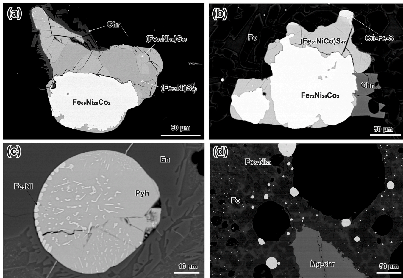
Fig. 3. BSE-images of the polished sections showing predominately sulfide and intermetallic phases. (a) Intermetallic compound \text{Fe}_{69}\text{Ni}_{29}\text{Co}_2 intergrown with Ni-bearing pyrrhotite in glass matrix of ICS slag; (b); (c) Intermetallic compound \text{Fe}_3\text{Ni} trapped in pyrrhotite (Pyh) embedded in enstatite crystal of IS slag; (d) overview micrograph showing smaller and bigger droplets of the intermetallic compound \text{Fe}_{77}\text{Ni}_{23} embedded in the enstatite-glass matrix, where magnesiochromite (Mg-chr) is also trapped.
