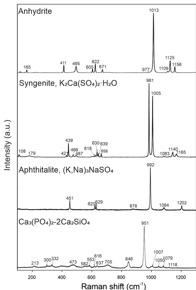
Fig. 6. Raman spectra of the mineral efflorescence on the seepage point of the CS samples and Raman spectrum of the \text{Ca}_3(\text{PO}_4)_2 \cdot 2\text{Ca}_2\text{SiO}_4 (CS slag).
