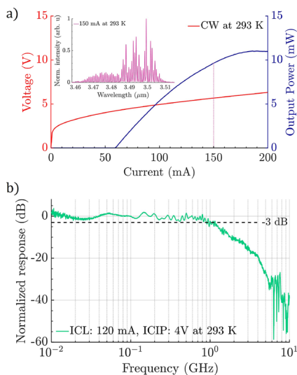
FIG. 2. (a) Light-intensity-voltage (LIV) curve of the ICL whose working wavelength is around 3.5 \mu\text{m} under continuous wave pumping at room temperature. The inset is the optical spectrum showing the wavelength of emission with a bias current of 150 mA at 293 K. (b) Normalized frequency response of the ICL when biased at 120 mA and with the ICIP biased at 4 V under 293 K, measured with a VNA.
