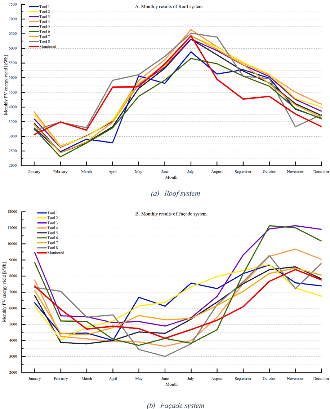
Fig. 5. Monitored and simulation monthly values of three systems.
