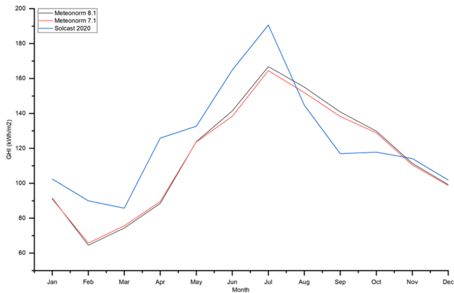
Fig. 3. Monthly GHI data comparison between measured data of Solacast for 2020 and Meteonom TMY.
