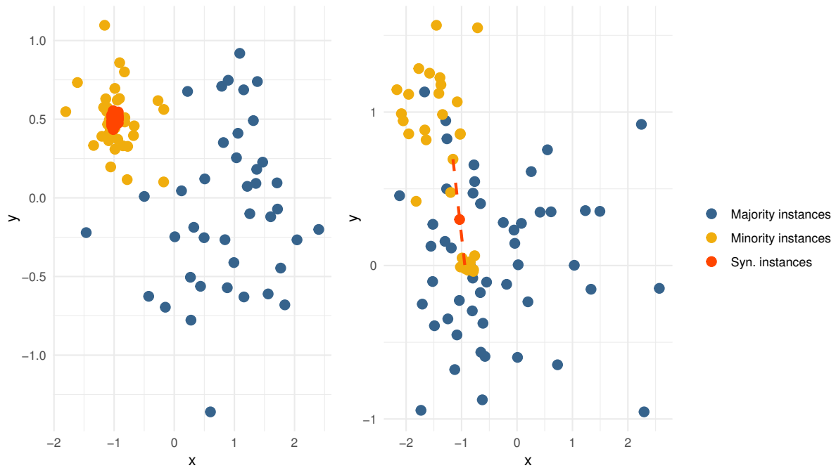
Figure 7: Dependency on k in SMOTE
