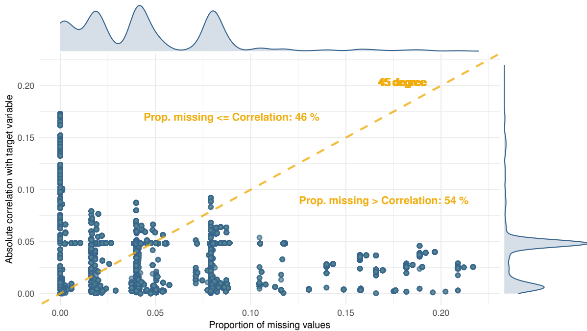
Figure 4: Proportion of missing values vs. absolute Pearson Correlation with target II
