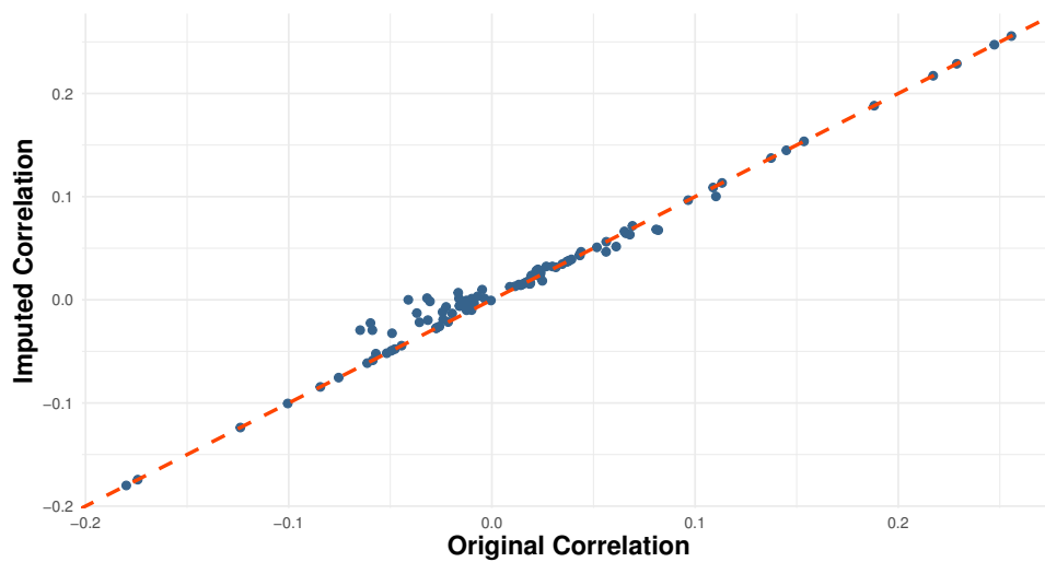
Figure 9: Correlation between the target variable and the imputed vs. original features
