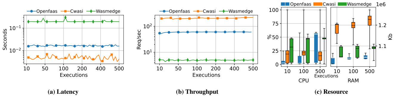
Figure 8: Fan-out Results
