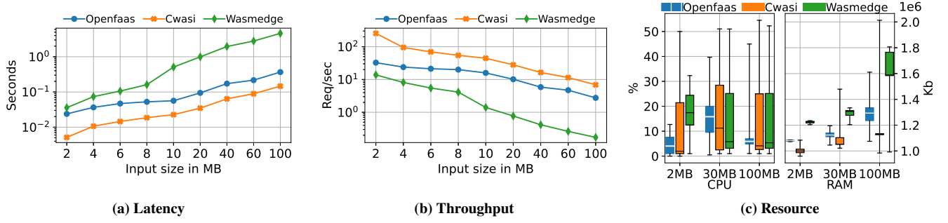
Figure 7: Sequential Results
