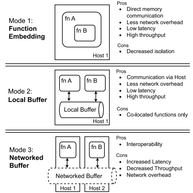
Figure 3: CWASI Inter-function Communication Model
