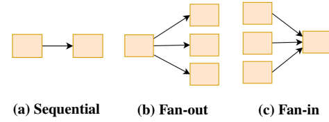
Figure 6: Experimental Workflows
