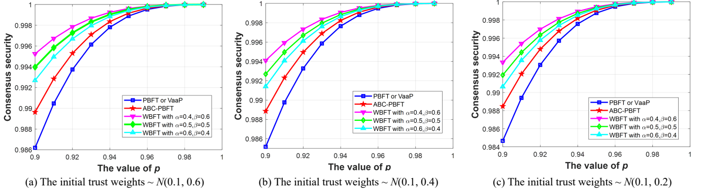
Fig. 4: Consensus security. (a) The initial trust weights of LLMs follow a N(0.1, 0.6) distribution. (b) The initial trust weights of LLMs follow a N(0.1, 0.4) distribution. (c) The initial trust weights of LLMs follow a N(0.1, 0.2) distribution.
