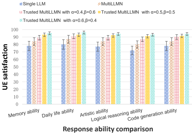
Fig. 8: UE satisfaction comparison.
