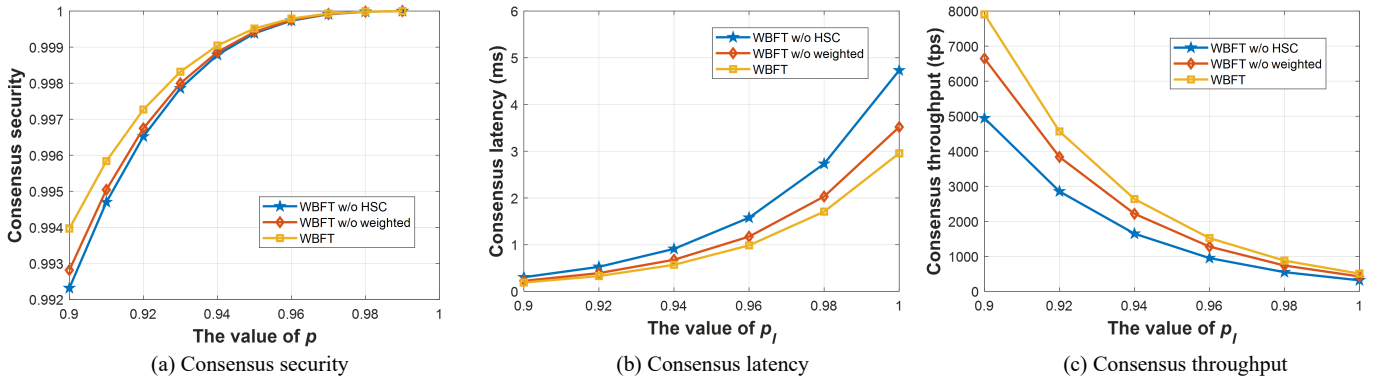
Fig. 7: Ablation test of WBFT when the initial trust weights follow a N(0.1, 0.6) with \alpha = \beta = 0.5 . (a) Consensus security. (b) Consensus latency. (c) Consensus throughput.
