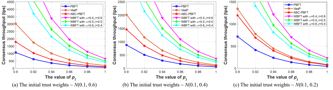
Fig. 6: Consensus throughput. (a) The initial trust weights of LLMs follow a N(0.1, 0.6) distribution. (b) The initial trust weights of LLMs follow a N(0.1, 0.4) distribution. (c) The initial trust weights of LLMs follow a N(0.1, 0.2) distribution.
