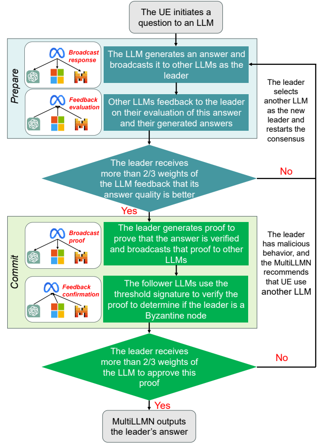
Fig. 3: The prepare and commit phases of WBFT consensus.
