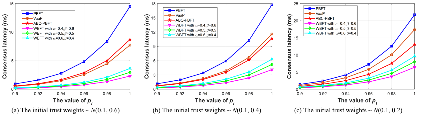
Fig. 5: Consensus latency. (a) The initial trust weights of LLMs follow a N(0.1, 0.6) distribution. (b) The initial trust weights of LLMs follow a N(0.1, 0.4) distribution. (c) The initial trust weights of LLMs follow a N(0.1, 0.2) distribution.
