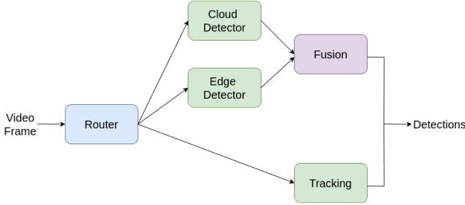
Fig. 1. VATE: A Compound AI System for Edge-Cloud Object Detection and Tracking. [7]
