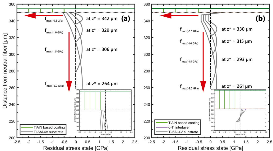
Fig. 10. Resulting residual stress gradients within the substrate for four different TiAlN top-coating stress states ( \sigma_{r,\parallel} = -0.5, -1.0, -1.5 and -2.0 \text{ GPa} , respectively, indicated by vertical green lines): (a) without (“No Interlayer system”) and (b) with a thin \alpha titanium interlayer (“Interlayer system”), determined by the linear-elastic stress-failure model. The neutral fiber (where \sigma_{K,a}(z) = 0 ) defines the origin of the model’s coordinate system. Insets in subplots (a) and (b) show magnified views of the residual stress gradient at the coating–substrate interface, altered by residual stress design. (For interpretation of the references to colour in this figure legend, the reader is referred to the web version of this article.)
