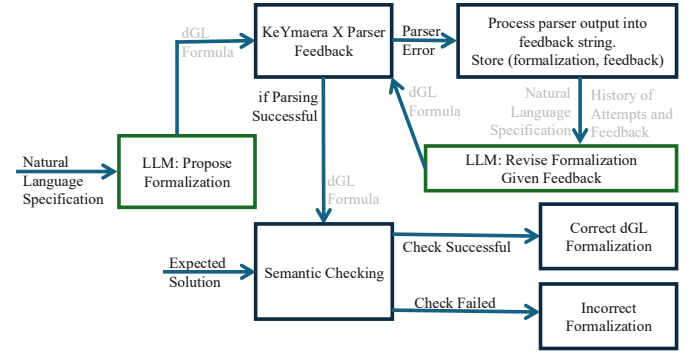
Fig. 1. Autoformalization pipeline
