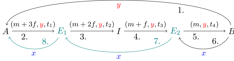
Figure 2.2: Wormhole Attack in Lightning.
