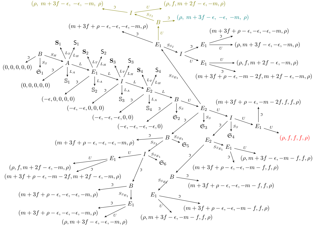
Figure 2.10: Partial Definition of the Lightning's Routing G_{\text{rout}} and the Fulgor Model G_{\text{Ful}} . The Olive Colored Subtree only applies for G_{\text{rout}} . The amount to be routed from player A to player B is m > 0 , and each of the intermediaries should receive a fee f .
