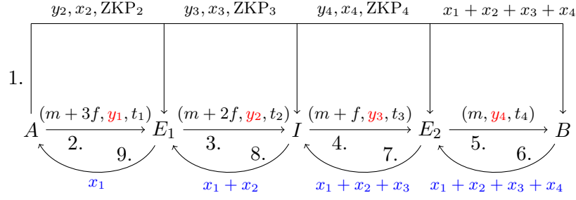
Figure 2.14: Routing in Fulgor.
